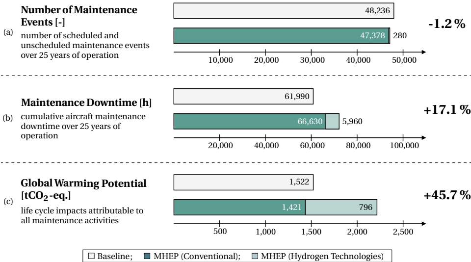
Figure 5.4: Comparison of the total number of maintenance events (a), total downtime due to maintenance (b), and overall environmental impact of all maintenance tasks (c) for the baseline (grey) and the MHEP (green) aircraft after an operating lifetime of 25 years. The light green area shows the respective share of the hydrogen technologies.
