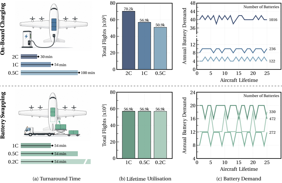
Figure 6.2: Schematic representation of the on-board charging and battery swapping turnaround strategies and the resulting turnaround times (a); aircraft utilisation over a 25-year operational lifetime for different turnaround strategies and charging scenarios (b); and annual battery demand over the aircraft lifetime resulting from battery degradation and additional battery sets required for battery swapping (c).
