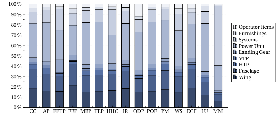
Figure 2.9: LCA results for the manufacturing phase across all impact categories.
