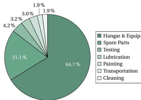
Figure 3.7: Distribution of the main drivers of the ecological implications.
