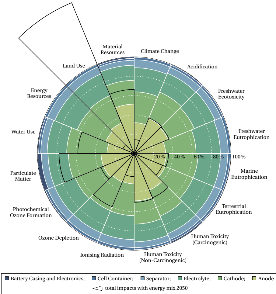
Figure 6.3: LCA results shown as a polar diagram across multiple midpoint impact categories based on EF 3.1.
