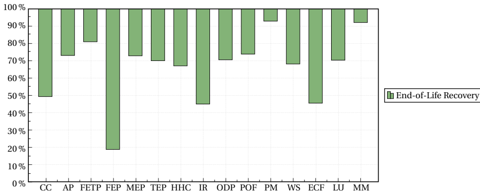
Figure 2.15: Ecological benefit due to the end-of-life phase (compared to the manufacturing phase) across all impact categories.
