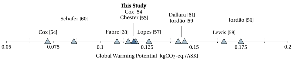
Figure 2.13: Comparison of the operations impact of this study with outcomes from other publications (normalised by ASK).
