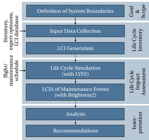
Figure 3.2: Process flow of the LCA approach.
