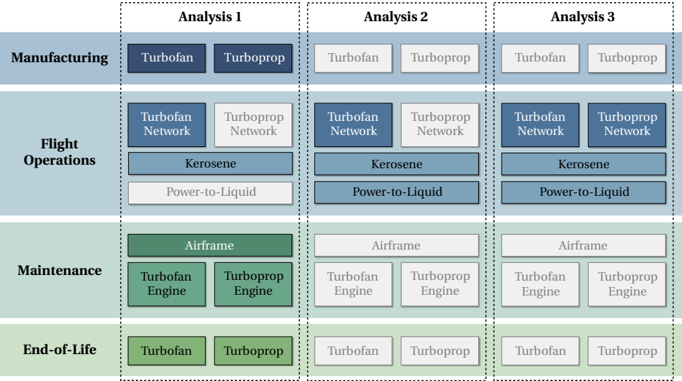
Figure 4.1: Graphical overview of the three analyses performed. The coloured boxes indicate what is included within the system boundaries of each analysis.
