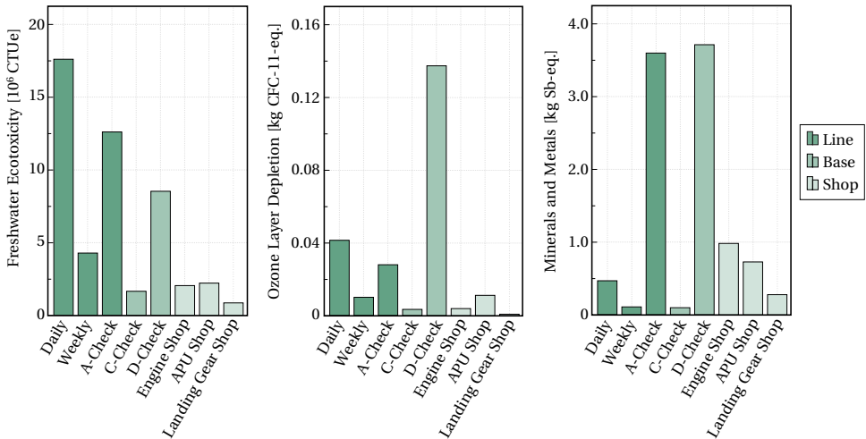
Figure 3.8: Comparison of LCA results for the impact categories FETP (left), ODP (middle), and MM (right). The bars are divided by colour into line, base, and shop maintenance.
