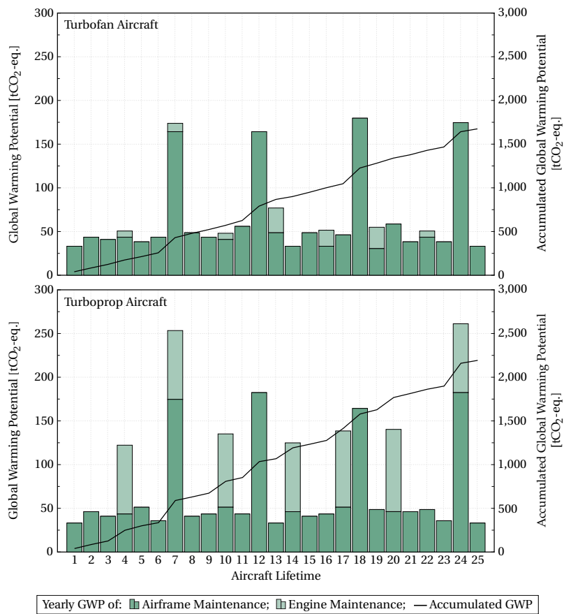
Figure 4.6: Yearly distribution of the GWP of the airframe and engine maintenance (primary axis) and the accumulative GWP of total maintenance over the turbofan (top) and turboprop (bottom) aircraft lifetimes (secondary axis).
