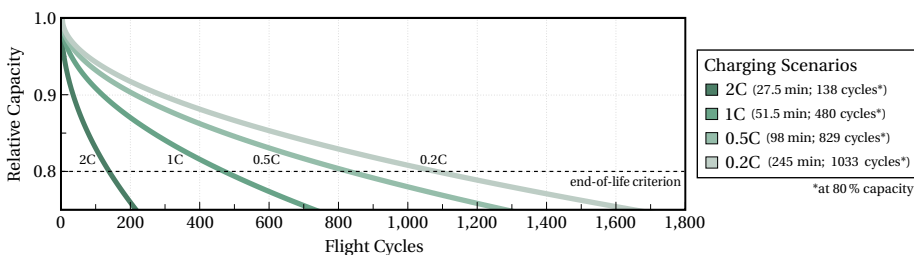
Figure 6.1: Relative battery capacity over FCs for charging scenarios ranging from 0.2C to 2C. The dashed line indicates the end-of-life criterion at 80 % remaining capacity.
