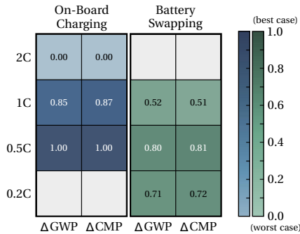
Figure 6.6: Normalised score (0 = least favourable, 1 = most favourable) for GWP and CMP, derived separately for each indicator across all scenarios. Hatched cells indicate scenarios that were not considered.
