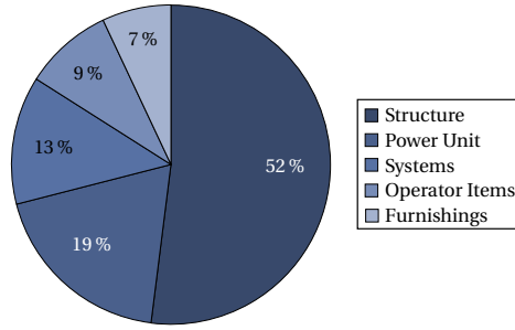
Figure 2.5: Mass breakdown of the considered aircraft based on CeRAS and own calculations and assumptions.
