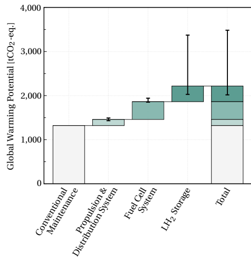
Figure 5.7: Waterfall diagram showing the GWP of all maintenance activities associated with the MHEP aircraft. The contribution of new hydrogen technologies is highlighted in green, and error bars represent the uncertainty in the maintenance impact.
