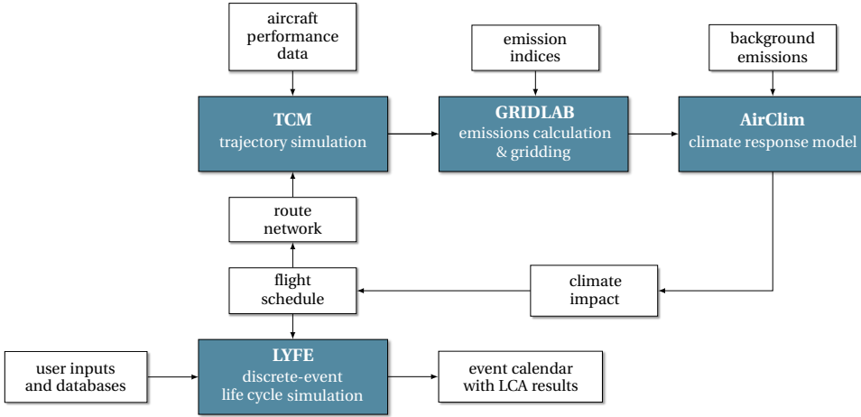
Figure 4.4: Schematic overview of the combined tools LYFE, TCM, GRIDLAB, and AirClim, including inputs and outputs.
