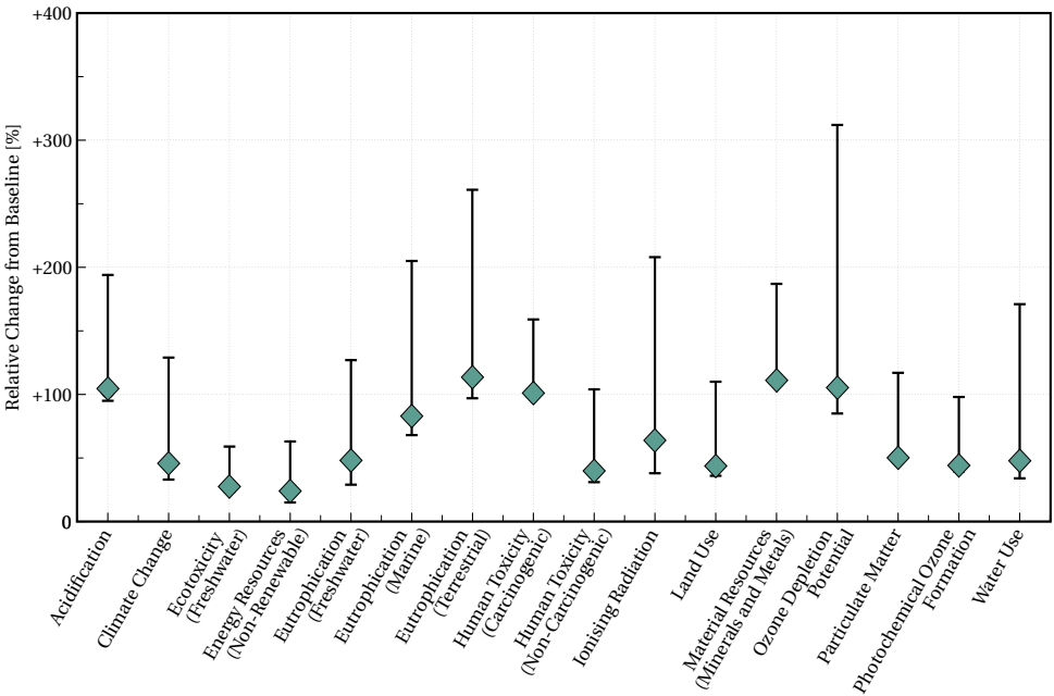
Figure 5.8: Deterministic LCIA results and uncertainty ranges for maintenance of the MHEP aircraft relative to the baseline aircraft (baseline = 0 %) across all EF 3.1 impact categories.
