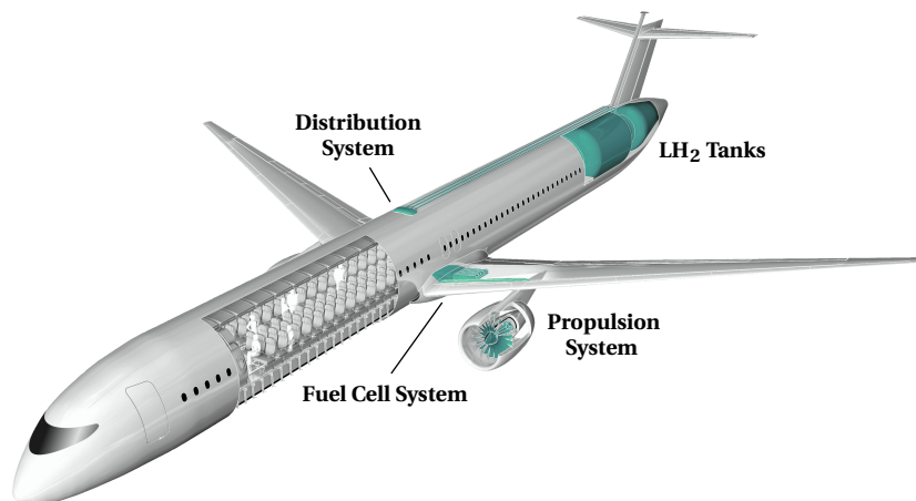
Figure 5.1: MHEP aircraft concept from the EXACT project. The two LH 2 tanks, the fuel cell system, and the advanced propulsion and distribution system are highlighted in green (source: DLR, internal documentation).
