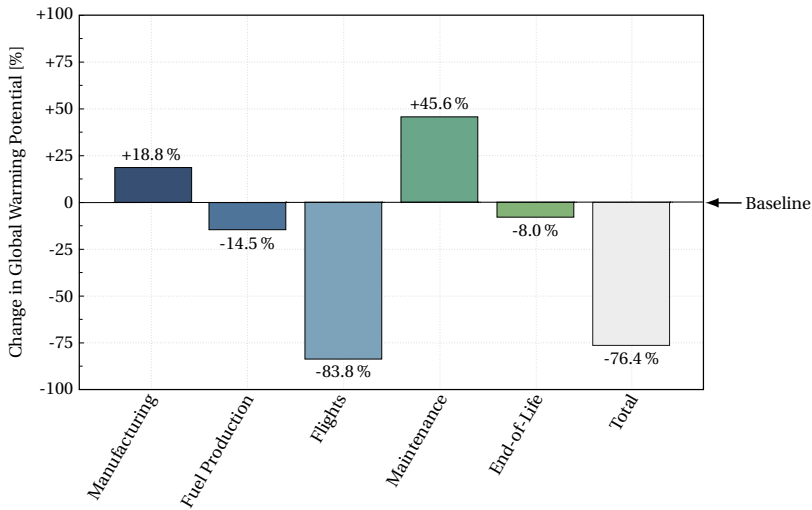
Figure 5.3: Changes in the GWP of the MHEP aircraft compared with that of the baseline aircraft for each life cycle phase. The total result indicates the overall GWP difference across all phases.
