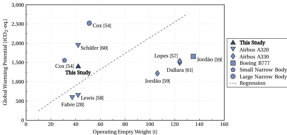
Figure 2.10: Overview of the GWP of this study and other publications over the associated OEW.
