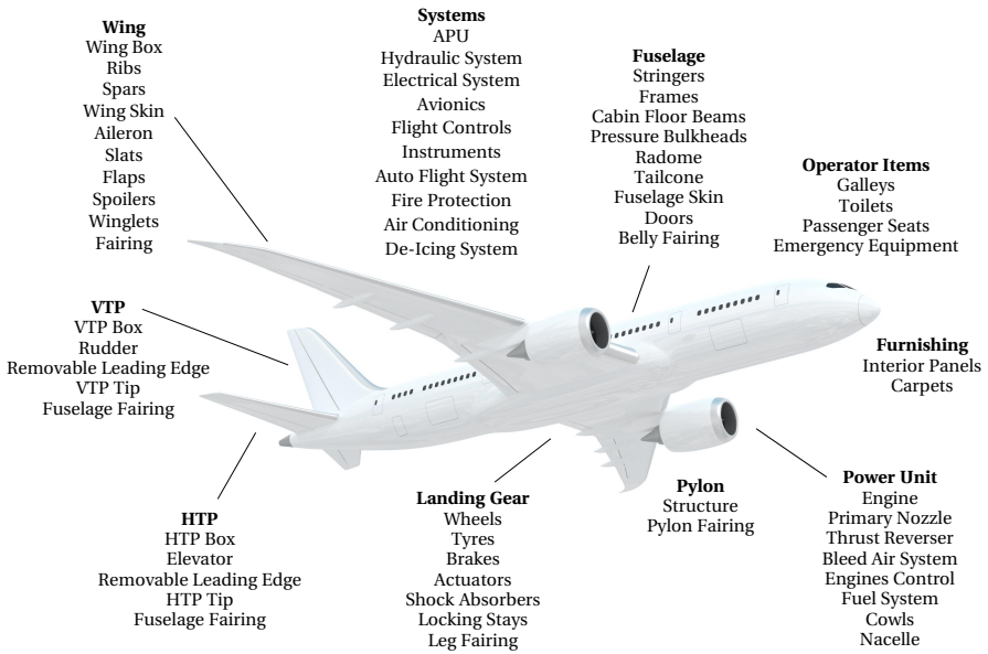
Figure 2.4: Component breakdown of the aircraft for the manufacturing LCI.
