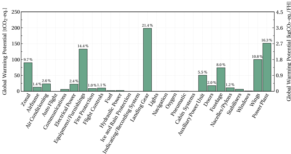
Figure 3.6: Comparison of the environmental impact of maintenance tasks for different ATA chapters in terms of absolute values and normalised per FH. The share of the total impact is additionally indicated for each component for which the contribution accounts for more than 1.0 % of the total share.
