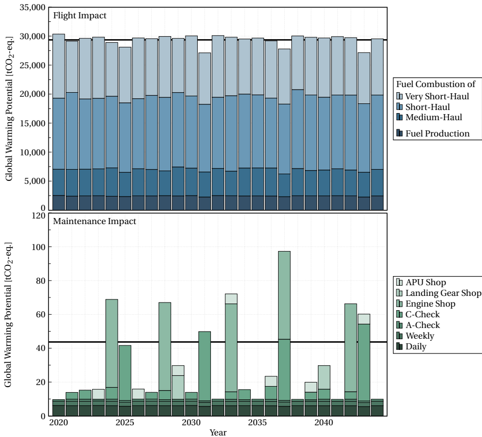
Figure 2.16: Effects of annually considered flight (top) and maintenance (bottom) events compared to usually on-average-determined ecological impacts (black line).
