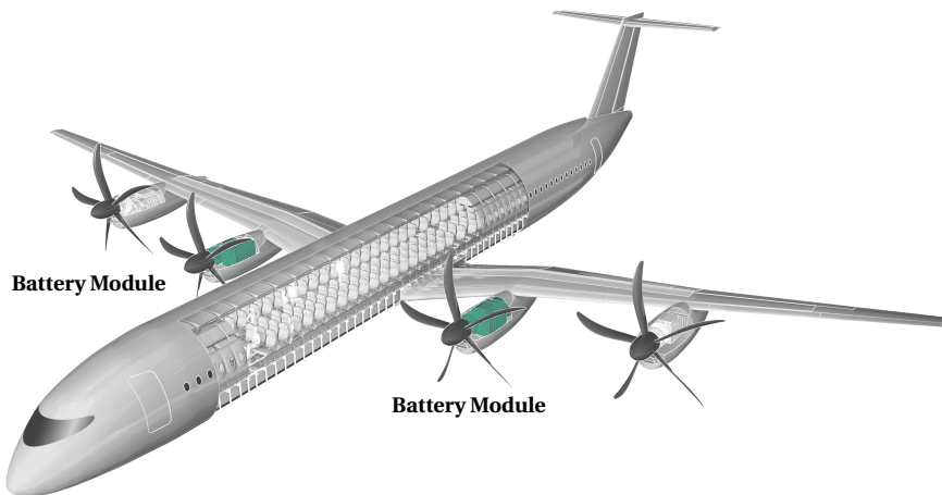
Figure 6.7: PHEP aircraft concept from the EXACT project. The two battery modules in the inner nacelles are highlighted in green (source: DLR, internal documentation).
