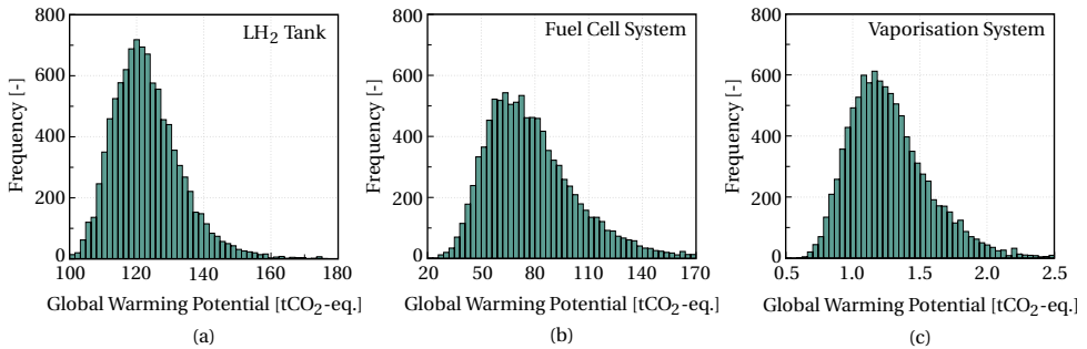
Figure 5.5: Uncertainty distribution of GWP results of the main replacement tasks: LH 2 tanks (a), fuel cell system (b), and vaporisation system (c), calculated using a Monte Carlo simulation with 10,000 runs.
