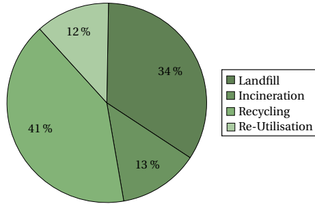
Figure 2.7: Distribution of the end-of-life scenarios of the entire aircraft based on the aircraft weight.
