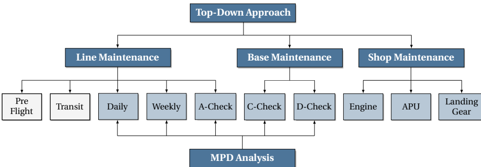
Figure 3.1: Overview of the combined methodology for the assessment of aircraft maintenance.
