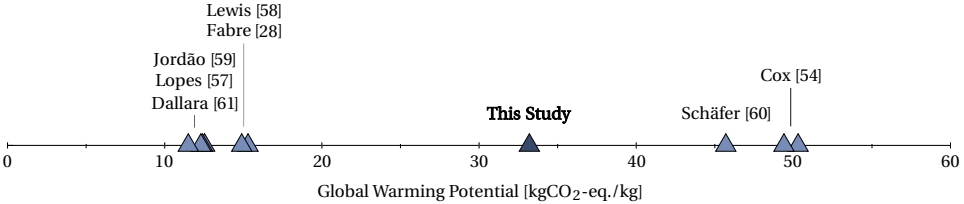
Figure 2.11: Comparison of the manufacturing impact of this study with outcomes from other publications (normalised by aircraft OEW).
