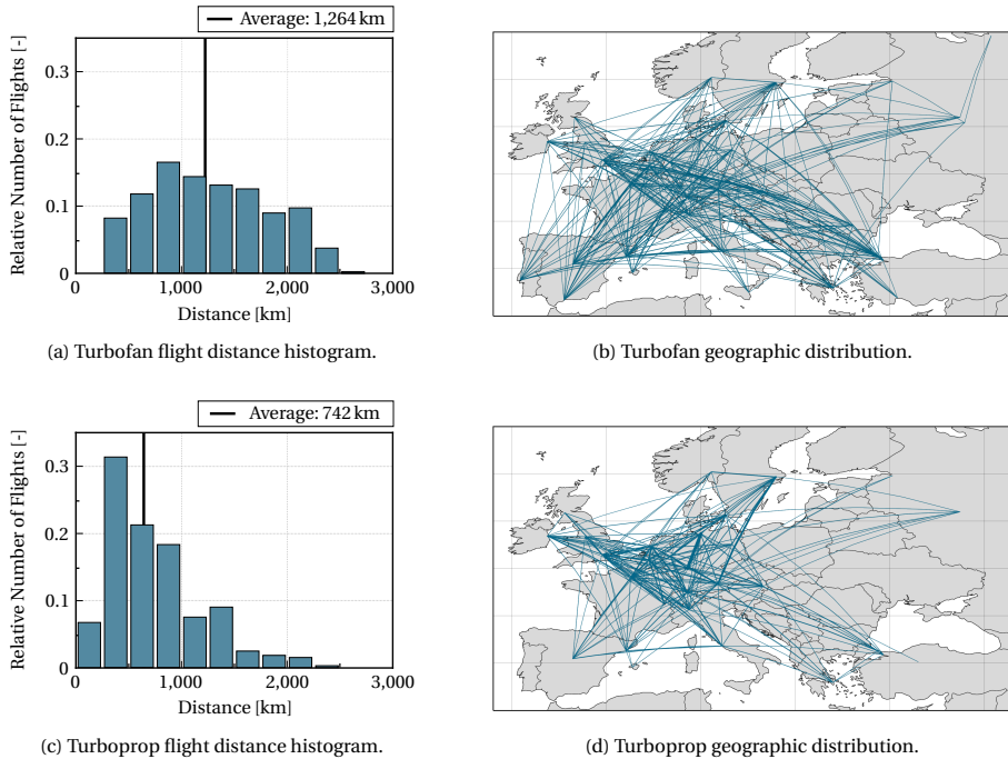
Figure 4.3: Flight distance histograms and geographical distributions of the two flight schedules.
