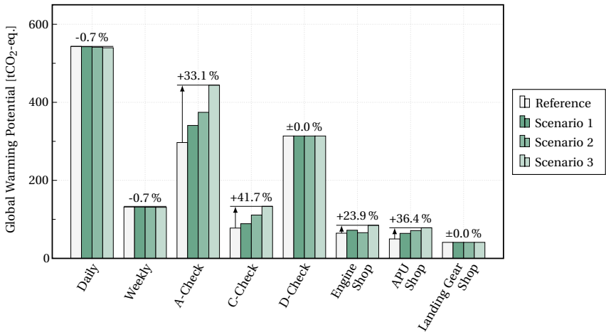
Figure 3.9: Overview of the ecological impact (given in GWP) including the largest deviation from the reference case for each scenario (Reference: FSNC/short-haul; Scenario 1: LCC/short-haul; Scenario 2: FSNC/long-haul; Scenario 3: LLC/long-haul).
