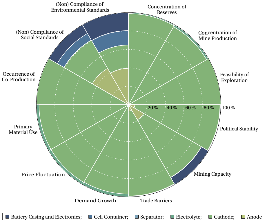
Figure 6.4: CA based on the ESSENZ methodology, illustrating supply risk and social impact indicators associated with the raw materials used in the battery module. The electricity mix is not a contributing factor to criticality and is therefore not represented in the polar chart.
