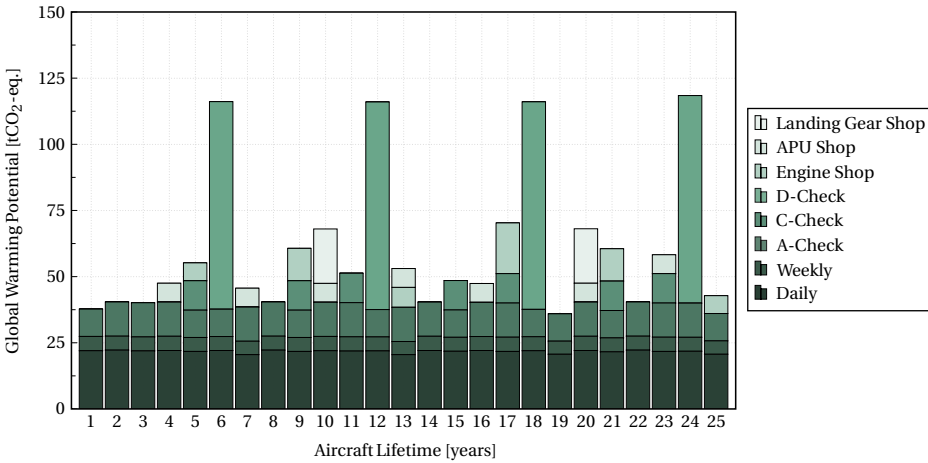
Figure 3.5: Distribution of maintenance-related environmental impact over the whole life cycle of the aircraft.
