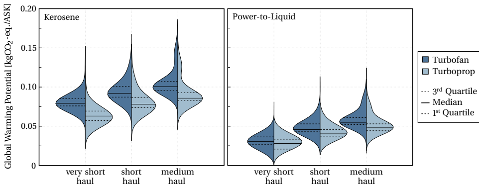
Figure 4.7: Distribution of the GWP results for the flight distance categories of very short-haul (up to 800 km), short-haul (800-1,500 km), and medium-haul (1,500-4,000 km) flights for kerosene (left) and PtL (right), including a comparison between turbofan and turboprop aircraft. The median and quartiles are shown in the violin plots to indicate the spread of the data.
