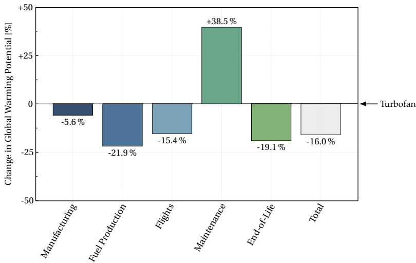
Figure 4.5: Changes in the GWP of the turboprop aircraft compared with that of the turbofan aircraft for each life cycle phase when powered with kerosene.
