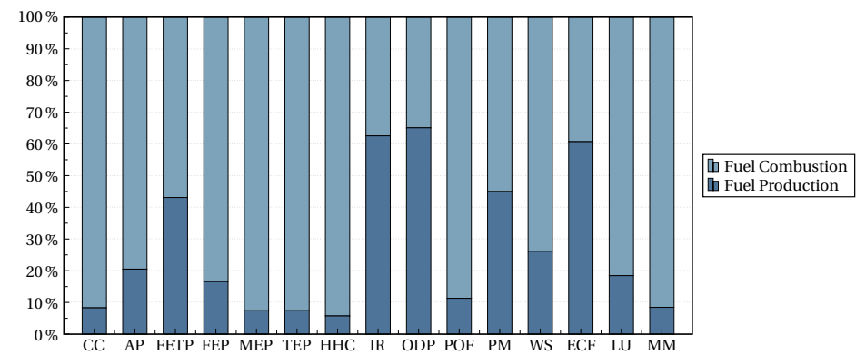
Figure 2.12: LCA results for the operation phase across all impact categories.
