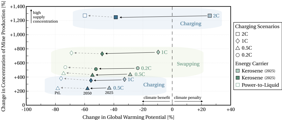
Figure 6.5: Change in GWP versus change in CMP for each charging scenario. The bottom-left region indicates combined climate and supply-risk benefits; the top-right a climate penalty and higher supply concentration. Marker shape denotes the charging scenario and the colour indicates the energy carrier. The arrows indicate the shift from kerosene (2025) to kerosene (2050) and further to PtL.
