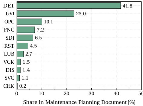
Figure 3.4: Share of task codes in the number of maintenance tasks in the MPD.
