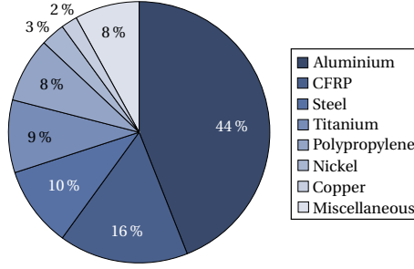
Figure 2.6: Material breakdown of the considered aircraft based on CeRAS and own calculations and assumptions.
