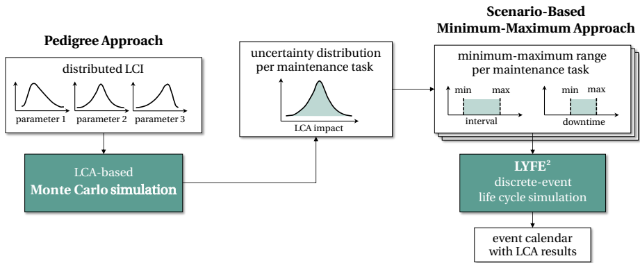
Figure 5.2: Schematic representation of uncertainty propagation: Task-level uncertainties are modelled using a Pedigree approach for each individual LCA, and operational uncertainties are captured via a scenario-based minimum-maximum approach for integration into LYFE 2 .
