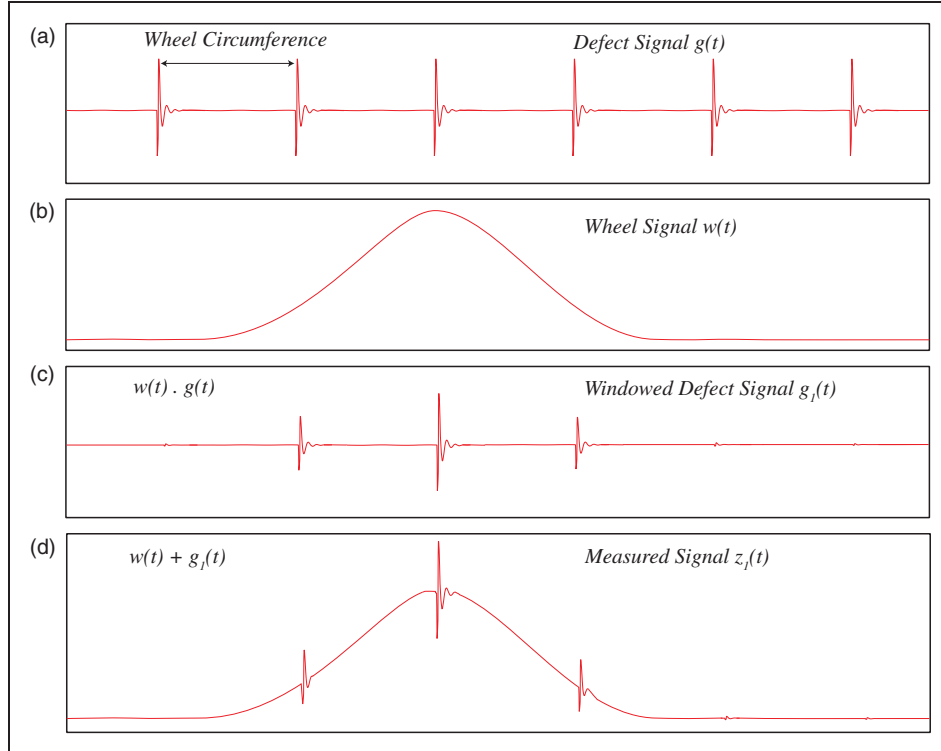
Figure 3. The schematic view of (a) the defect signal g(t) , (b) the wheel signal w(t) , (c) the windowed defect signal g_1(t) , and (d) the measured signal z_1(t) .
