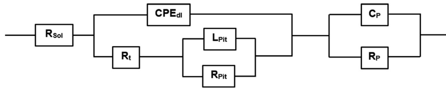
Fig. 9 – Obtained equivalent circuit diagram of the fitted EIS data by using the ZsimpWin 3.21 software.
