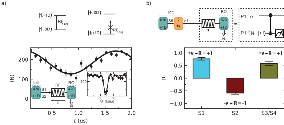
Figure 4.5: Nitrogen nuclear spin control and NV-P1 coupling sign. a) ^{14}N Rabi oscillation. Top: energy levels of the P1 electron spin in the \{0D, +1D\} subspace. Bottom: either S1 or S2 is prepared in |+1, D\rangle and the length t of a pulse at frequency RF = RF_{14N} = 36.8 MHz is varied. The nitrogen nuclear spin is driven conditionally on the electron spin state. Inset: NMR spectrum obtained by varying the frequency RF for a fixed pulse duration t . b) We use the ^{14}N spin to determine the sign of the NV-P1 coupling. First, we prepare a selected P1 center ( K=820 ) and initialise its electron spin ( L=2 ). Second, we apply a \pi pulse at RF_{14N} , which implements an electron controlled CNOT e,N (see level structure in (a)). The coupling sign to the NV determines the P1 electron-spin state, and, in turn, the final ^{14}N state. Finally, we measure the fidelity with the ^{14}N |+1\rangle state for two opposite electron spin initialisations ( +y and -y final \pi/2 pulse of DEER( y )). The normalized difference R of these measurements reveals the sign of the coupling (see Methods). All error bars indicate one statistical standard deviation.
