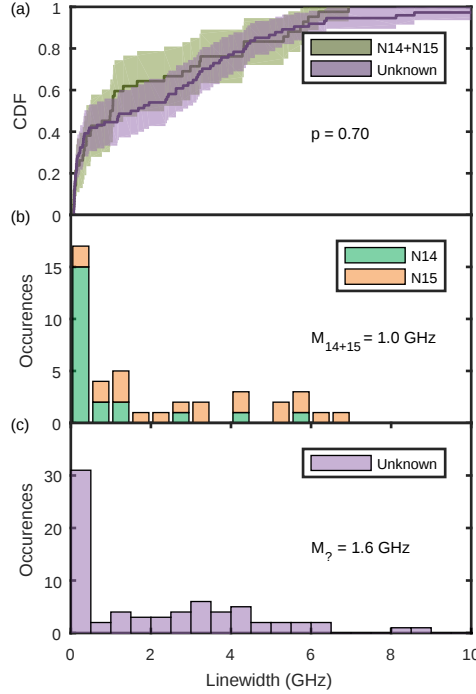
Figure 3.6: Summary of all data for sample A. (a) A CDF representing the distributions of unknown isotope to known isotope ZPL linewidths. A similar shape indicates that both sample sets are drawn from the same distribution indicating there is no inherent bias towards sampling ^{14}\text{NV} or ^{15}\text{NV} . The probability to obtain these results if the samples are drawn from the same distribution ( p ) is evaluated by a Wilcoxon rank-sum test. (b) A stacked histogram showing all the ^{14}\text{NV} and ^{15}\text{NV} ZPL linewidths. The median linewidth ( M ) is indicated. (c) A histogram showing the linewidths for the set of ZPLs with an unknown host isotope.
