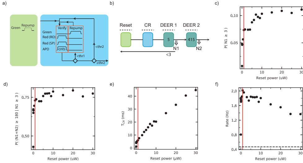
Figure 4.15: Active optical reset of P1 bath. a) Illustration of the green (515 nm) optical reset pulse (left). Logical sequence showing the charge and resonance verification (CR) for the NV center (right). We count the number of photons (cnts) while resonantly exciting the NV center simultaneously at its readout (RO) and spin-pump (SP) transitions. If \text{cnts} < \text{thr1} , the charge state is optically reset (repump, 30 \mu\text{W} ). The experimental sequence is continued if \text{cnts} \geq \text{thr2} ( \text{thr2} > \text{thr1} ). If \text{thr1} \leq \text{cnts} < \text{thr2} , a new verification step is entered. b) Schematic of the experimental sequence. An initial optical reset is performed (green, 5 \mu\text{s} ) to excite the P1 bath [70]. Thereafter, the CR scheme (blue, see (a)) is implemented until the experimental sequence is continued. This scheme is followed by a DEER sequence ( K=5 , see main text). Based on the outcome of DEER 1 we either continue to DEER 2 ( K=415 ) or go back to the start of the experimental sequence to apply an optical reset pulse. c), d) Plots of the probabilities to pass the desired threshold after DEER 1 and DEER 2, as a function of the optical reset pulse power. e) Average duration of the CR scheme ( T_{CR} ) as a function of optical reset pulse power. f) Experimental rate given the desired threshold ( N1 + N2 \geq 180 ). The dashed horizontal line marks the rate without optical reset pulse and without feedback based on the outcome N1 . Vertical red lines in c), d), e), f) mark the reset power for maximal experimental rate.
