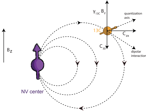
Figure 5.3: ^{13}\text{C} spin in a dipole field. Exemplary case in which the J_z I_x interaction causes its quantization axis to become more aligned with the dipole field direction due to the the NV ( m_s = -1 ) given the condition C_{zz} < \gamma_{13\text{C}} B_z . The same holds for the NV in m_s = +1 , in this case the direction of the dipole field and thus C_{zx} and C_{zz} change to their direct opposite.
