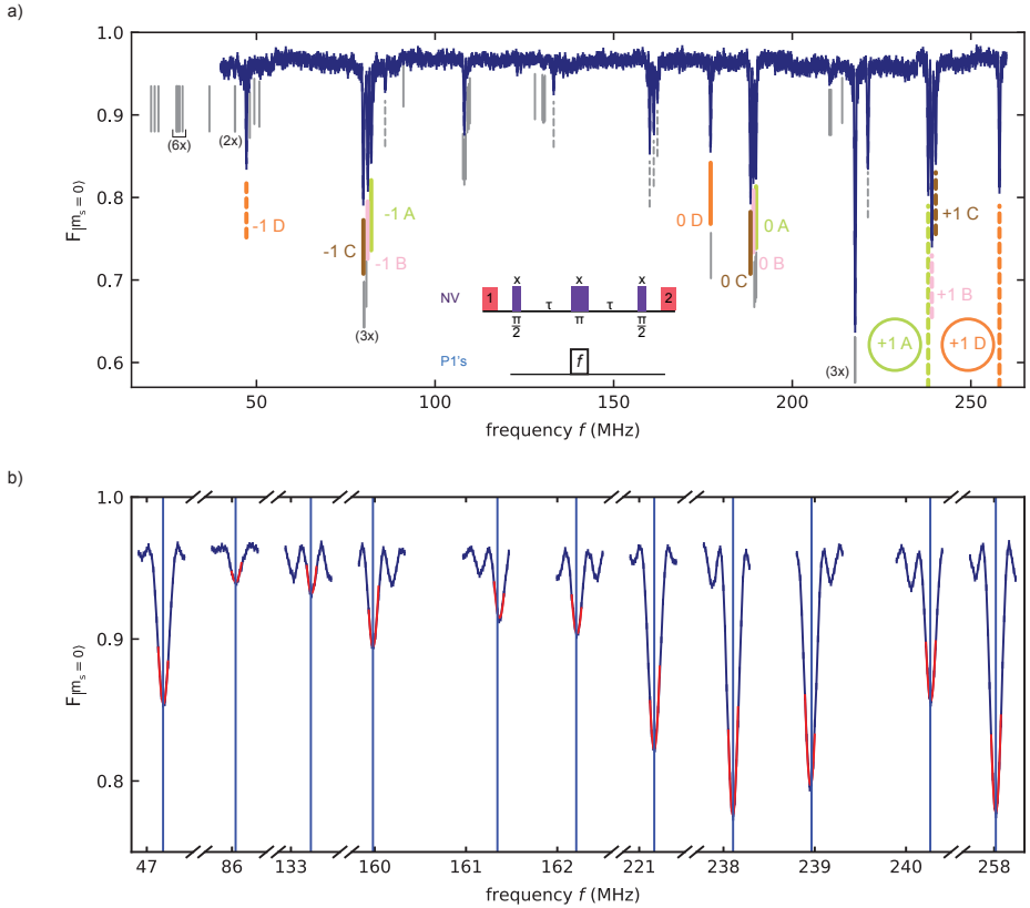
Figure 4.9: Fitting the P1 Hamiltonian parameters. a) Complete dataset corresponding to Fig. 4.1b (main text). b) Measurement of 11 dips that are assigned to a well isolated transition (blue lines). Side lobes are due to Rabi oscillations. We fit a parabola (red) and extract the center frequency. Using a least squares fit of the center frequencies and the transitions, we extract the values of \{A_{\parallel}, A_{\perp}, P_{\parallel}\} and \vec{B} . Error bars indicate one statistical standard deviation, with a typical value 2 \times 10^{-3} , which is smaller than the data points.
