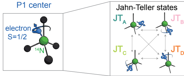
Figure 2.5: P1 center in diamond. Left: the P1 center surrounded by four carbon atoms in the diamond lattice. Right: the P1 center exhibits a Jahn-Teller distortion along one of the four 14 N - C bonds (labelled as {A,B,C,D}) that can vary over time.
