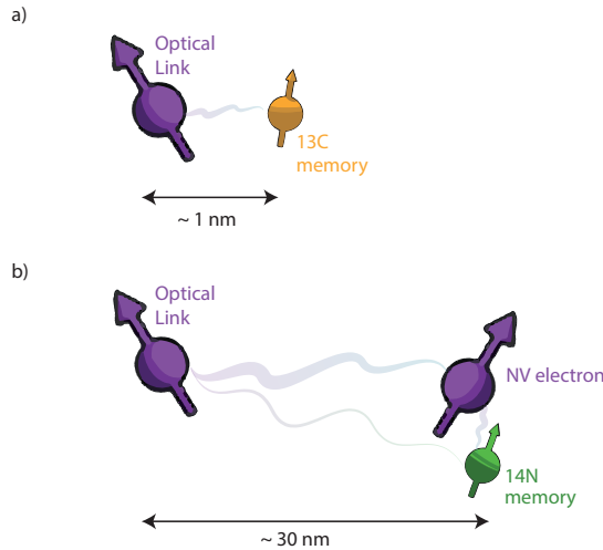
Figure 5.8: Quantum memories. a) ^{13}\text{C} spin (memory) coupled to an NV center that is used as an optical link (communicator). b) System of coupled NV centers. At \sim 30 nm, the ^{14}\text{N} nuclear spin (memory) is accessible indirectly via a relatively strong ( \sim\text{kHz} ) electron-electron coupling between NV electrons. The ^{14}\text{N} spin is also robust against undesirable changes of the electron state of the optical link NV center (communicator), as the electron-nuclear coupling is much weaker (sub-Hz).
