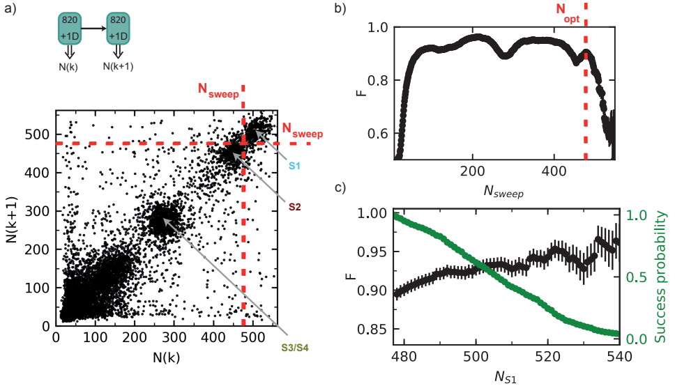
Figure 4.20: Optimization of combined initialisation and readout of S1 in |+1, D\rangle . a) Full correlation plot for consecutive measurement outcomes N(k) and N(k+1) , both for |+1, D\rangle (same dataset as Fig. 4.3a in the main text). We set the thresholds N_{S1} = N_{notS1} = N_{RO} all equal to N_{sweep} (see main text Fig. 4.3a). Using these thresholds we calculate F as in eq. 4.31 for different values of N_{sweep} . b) Fidelity F as a function of N_{sweep} . The red dashed line indicates a local maximum of F (here N_{sweep} = N_{opt} = 477 ) that optimally separates between S1 and S2 under the given constraints ( N_{S1} = N_{notS1} = N_{RO} = N_{sweep} ). The same value ( N_{sweep} = N_{opt} ) is shown by the red dashed lines in (a). c) Further improvement of F at the cost of experimental rate is achieved by a stricter initialisation threshold N_{S1} . First we set N_{notS1} = N_{RO} = N_{opt} and vary N_{S1} . The fidelity F is plotted as function of N_{S1} (black). The success probability of initialisation of S1 in |+1, D\rangle as compared to when N_{S1} = 477 is plotted in green as a function of N_{S1} .
