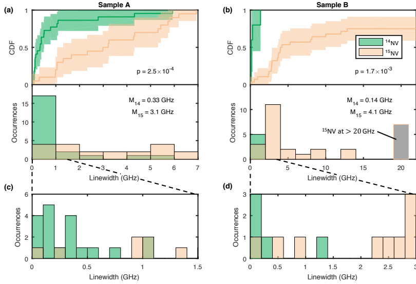
Figure 3.3: Optical linewidths per isotope. a-b , A summary of the optical linewidths identified in sample A ( a ) and sample B ( b ) from scans at the implantation depth. For sample B, that has comparatively few ^{14}\text{NV} centers at the implantation depth, we included three ^{14}\text{NV} centers found deeper in the diamond to enable a comparison between NVs formed from implanted versus native nitrogen. The distribution is represented as a cumulative distribution function (CDF, top), with the corresponding histogram shown below. The shaded region in the CDF indicates a 95% confidence interval calculated using Greenwood's formula. These data show that both diamonds supported narrow-linewidth NV centers, the majority of which originated from ^{14}\text{NV} s. While ^{15}\text{NV} do exhibit narrow lines, their median linewidth ( M ) is higher than for the ^{14}\text{NV} centers in both samples. We evaluate the probability to obtain the observed linewidths for ^{14}\text{NV} centers and ^{15}\text{NV} centers if the samples are drawn from the same distribution with a Wilcoxon Rank Sum test, finding a p-value of 2.5 \times 10^{-4} in sample A and 1.7 \times 10^{-3} in sample B. c-d , A magnification of the histograms shown in a and b .
