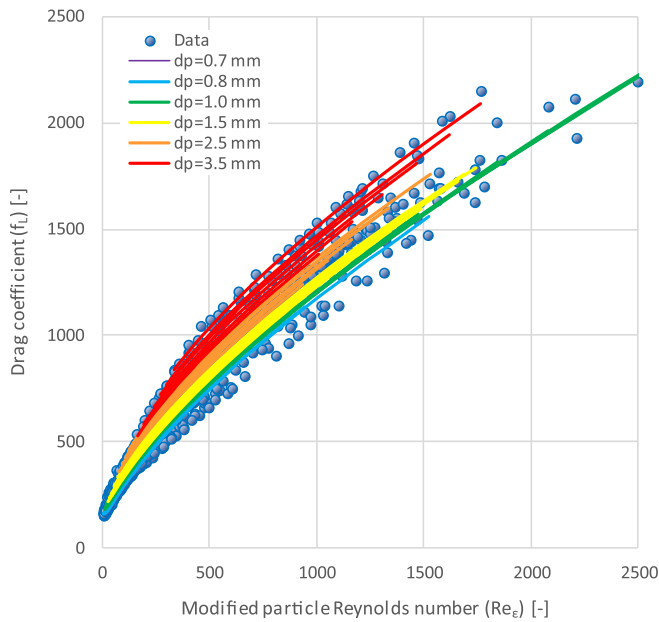
Fig. 11. Drag coefficient f_L versus Re_e for glass beads and RIO 1 model (highest R^2 ).
