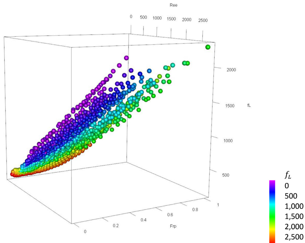
Fig. 10. Rotated 3D plot ( f_L versus Re_\varepsilon , Fr_p ) based on experimental data (calcite pellets) in the fluidised state.
