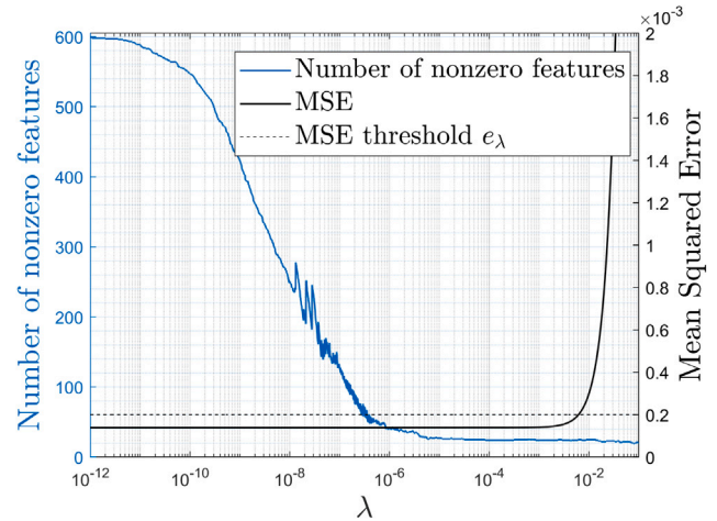
Fig. 6. Mean Squared Error and number of non-zero features vs. \lambda with noise \sigma = 1 \times 10^{-2} mm.
