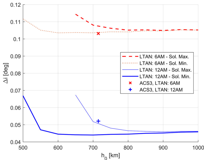
Fig. 22. Inclination increase steering law: inclination increase for a_c = 5 \cdot 10^{-2} mm/s 2 .
