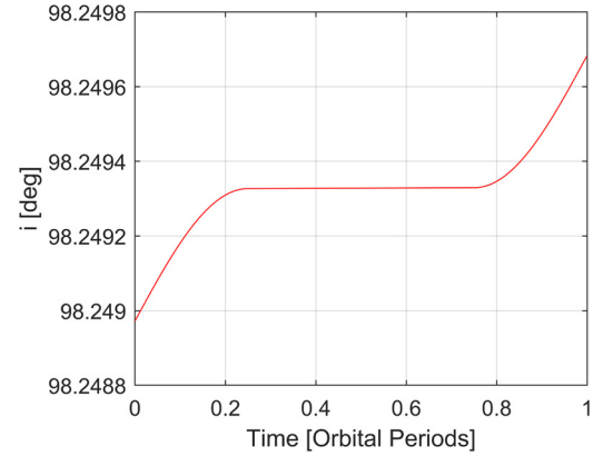
Fig. 14. Inclination increase: variation in inclination of the POINT solution over one orbital period.
