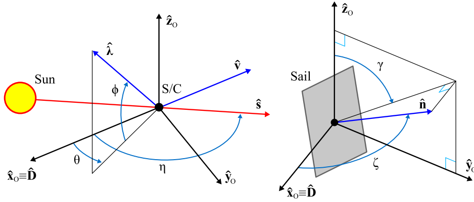
Fig. 3. Optimization reference frame, O_0(\hat{x}_0, \hat{y}_0, \hat{z}_0) .
