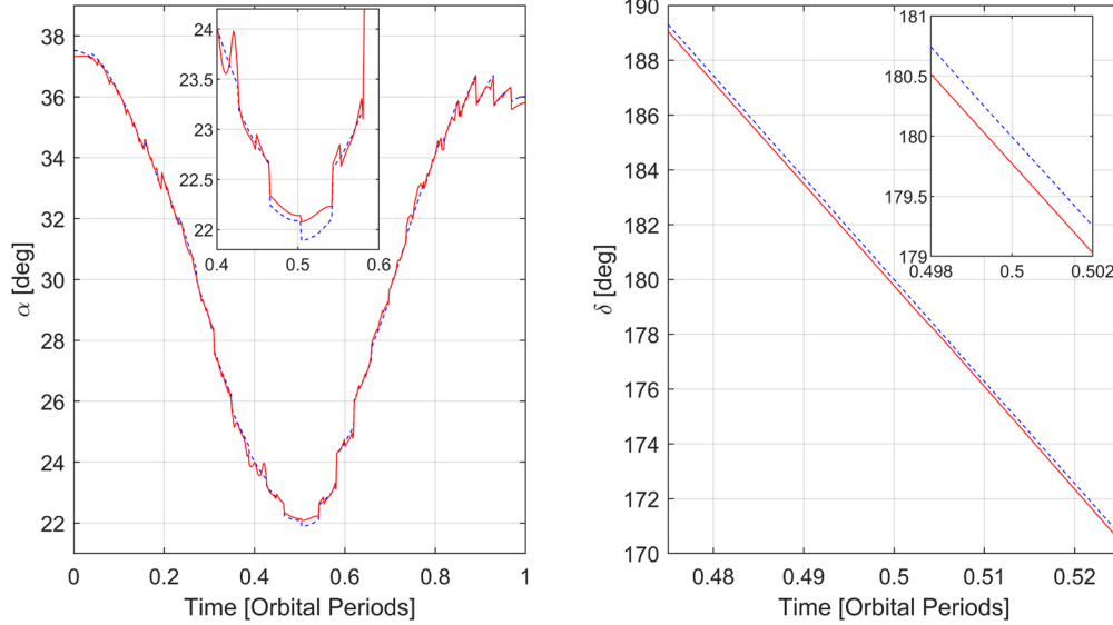
Fig. 8. Orbit raising: control profile of the reference solution (blue, dashed) and POINT solution (red, solid) over one orbital period.
