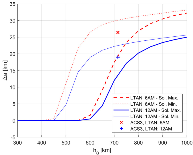
Fig. 20. Orbit raising steering law: SMA increase for a_c = 5 \cdot 10^{-2} mm/s 2 .
