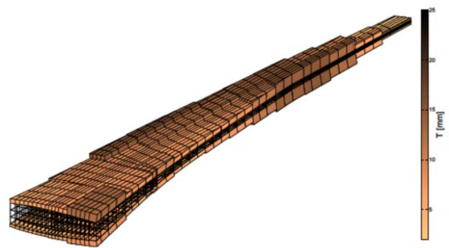
Figure 9: Typical resulting thickness distribution of laminates after wing optimization
