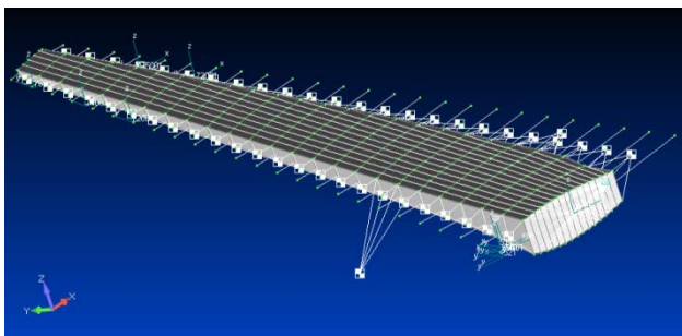
Figure 11: Structural layout of the NSR wing box
