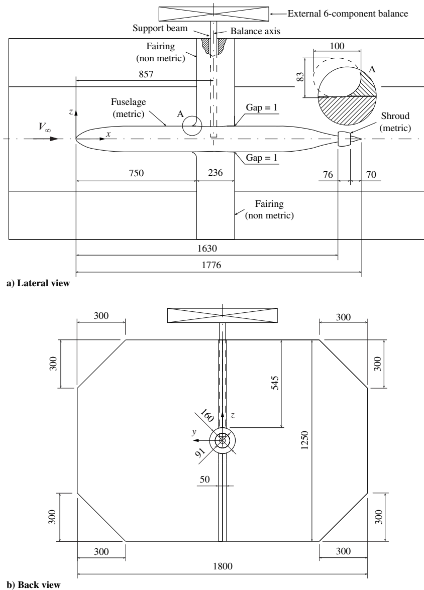
Fig. 2 Technical drawing of the wind-tunnel setup used during the experiments in the Low Turbulence Tunnel of Delft University of Technology. (Dimensions are in millimeters.)
