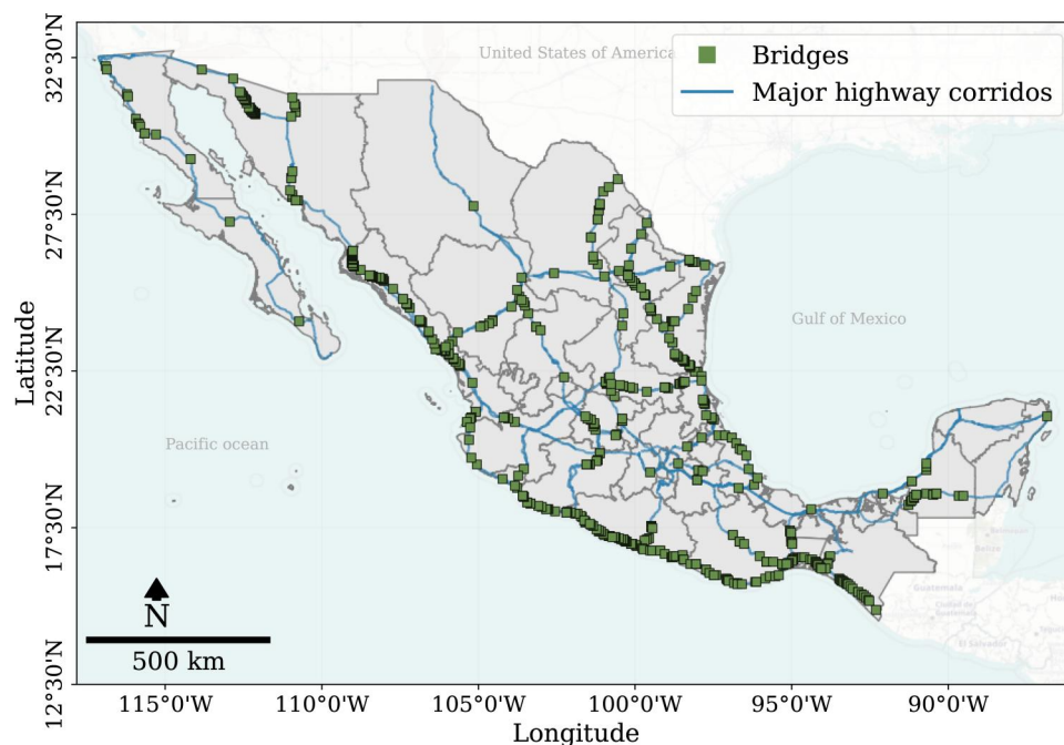
Figure 4. Location of the bridges under study.
