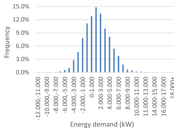
Fig. 7 Frequency (per 0.1 s) per energy demand interval
