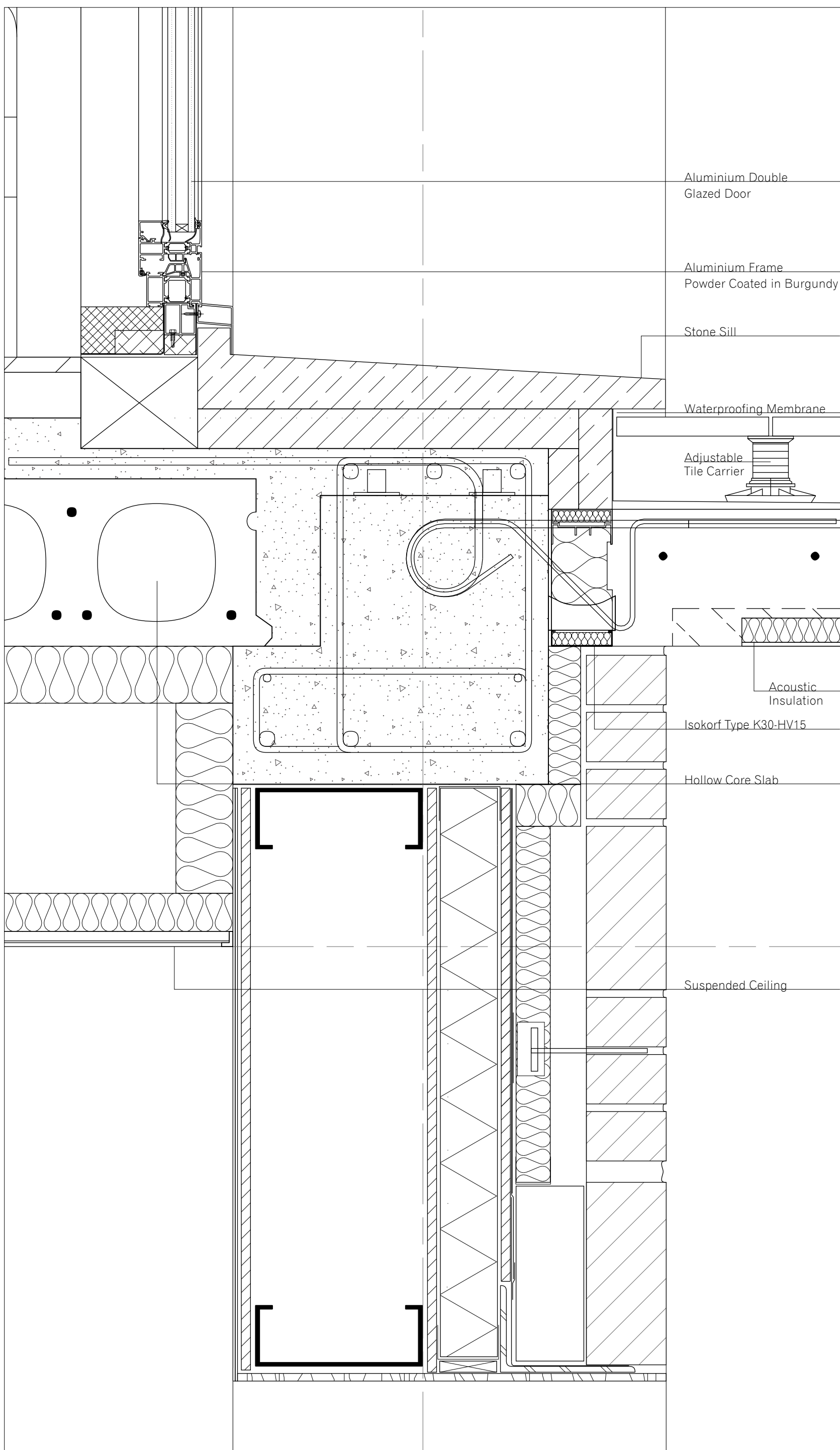
DETAIL SECTION 1 SCALE 1:5
