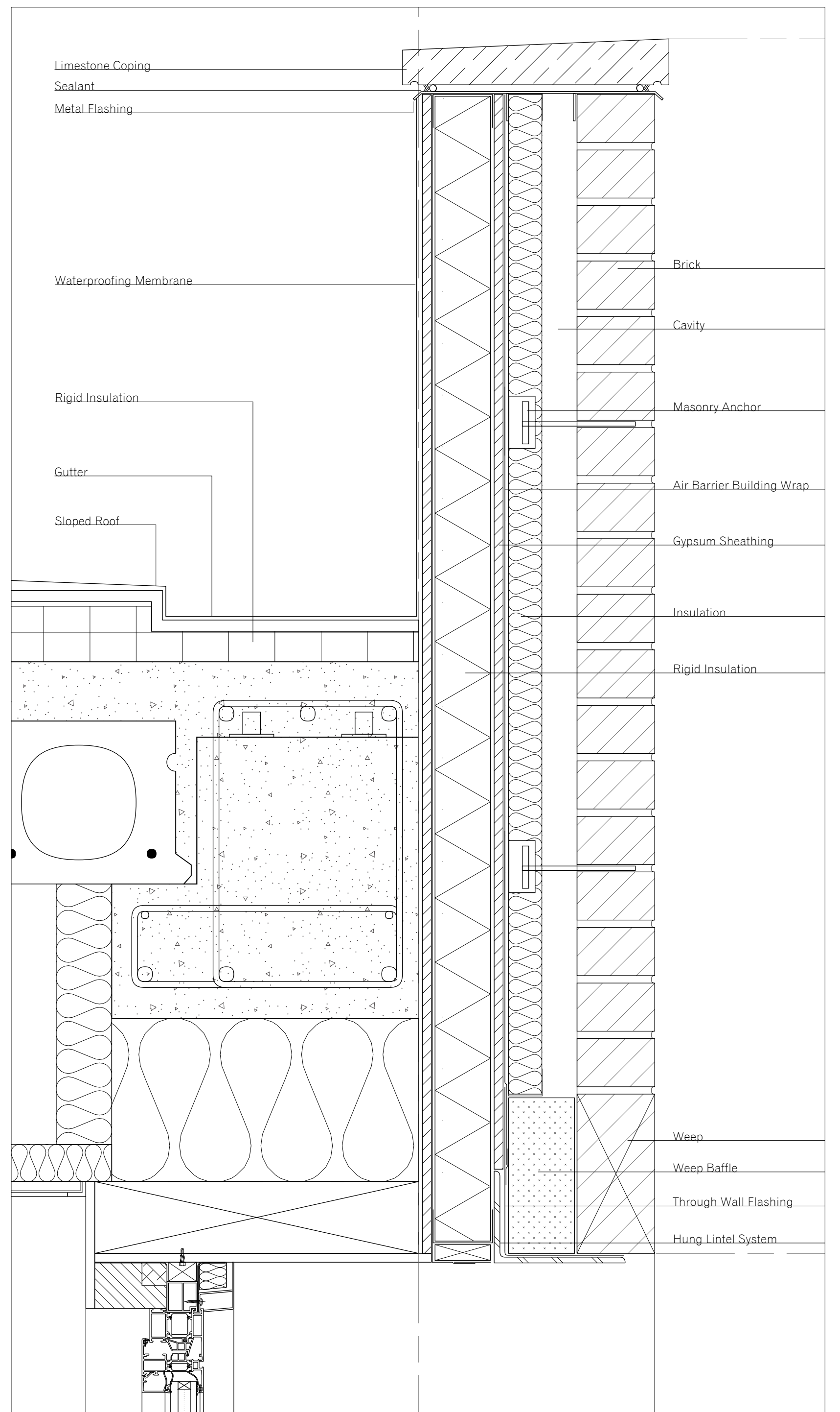
DETAIL SECTION 2 SCALE 1:5
