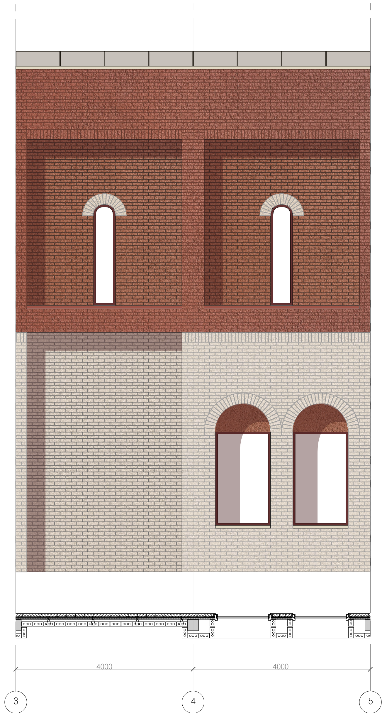
FACADE DETAIL SCALE 1:50
