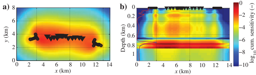
Figure 4. (a) Depth slice at reservoir level (785 m) of the normalized cumulative sensitivity to vertical resistivity. (b) Depth section of normalized cumulative sensitivity at y = 4 km. The black lines indicate the positions of the sources, and the black triangles indicate the positions of the receivers. As a reference, the 1D horizontal and vertical resistivity profile of Figure 2 is plotted on the left.
