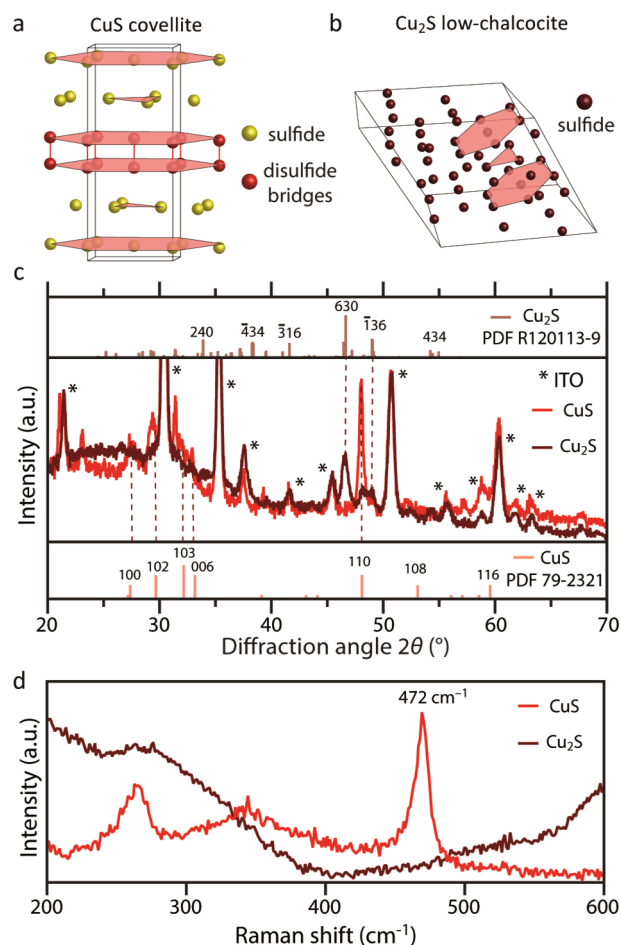
Figure 5. Phase transformation of covellite CuS into low-chalcocite \text{Cu}_2\text{S} . (a) Model showing the covalent S–S bond and hcp anion sublattice in covellite CuS. (b) Model showing hcp anion sublattice of low-chalcocite \text{Cu}_2\text{S} . (c) XRD measurements of CuS NCs before (red line) and after (brown line) electrochemical charging in the presence of \text{Cu}^+ ions. The XRD pattern of the CuS NCs shows the characteristic (110) reflection for covellite, whereas the XRD pattern after electrochemical charging clearly shows the (630) reflection of low-chalcocite \text{Cu}_2\text{S} . Reference bars are from PDF cards 79–2321 and R120113–9 for covellite CuS and low-chalcocite \text{Cu}_2\text{S} , respectively. (d) Raman spectrum for a film of CuS NCs (red line), showing the characteristic S–S stretching mode at 472 \text{ cm}^{-1} , and Raman spectrum for a film of \text{Cu}_2\text{S} NCs (brown line), in which no disulfide bridges are observed at 472 \text{ cm}^{-1} , indicating successful reduction of the anionic sublattice.
