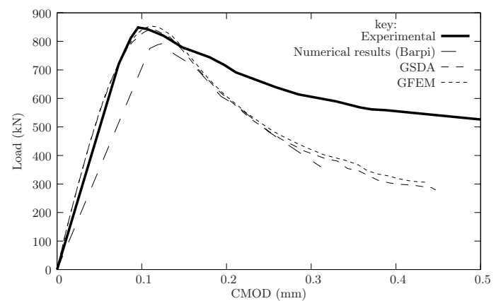
Figure 7. Prenotched gravity dam model: load vs. CMOD.
