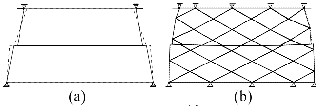
Figure 5. Deformed mesh (reduced 10\times ) for the GSDA (continuous) and the GFEM (dashed): (a) one finite element; (b) distorted non-symmetric mesh.
