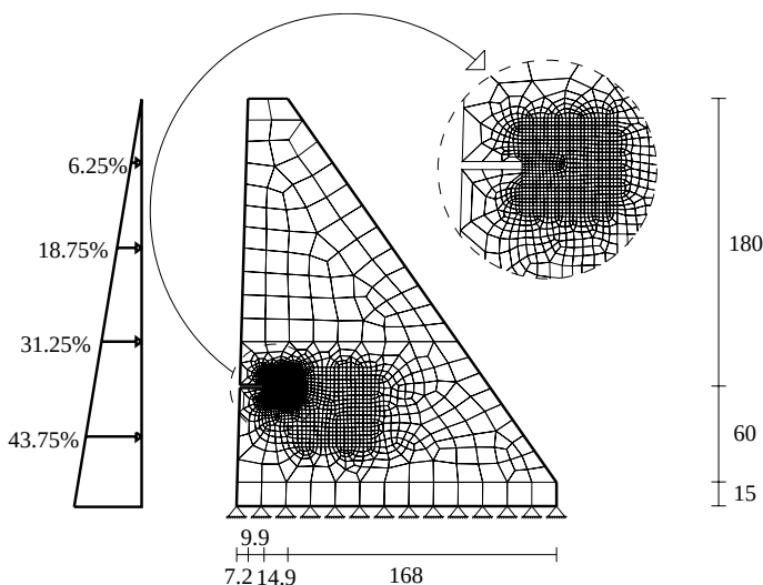
Figure 6. Prenotched gravity dam model: structural scheme (thickness 30 cm), including loading, boundary conditions and adopted mesh (all dimensions in cm).
