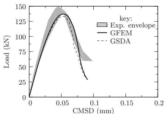
Figure 11. Four-point shear test: load vs. CMSD.
