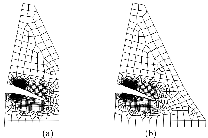
Figure 9. Prenotched gravity dam model: deformed mesh (magnified 500\times ) when CMOD is 0.35 mm for: (a) GSDA; and (b) GFEM.
