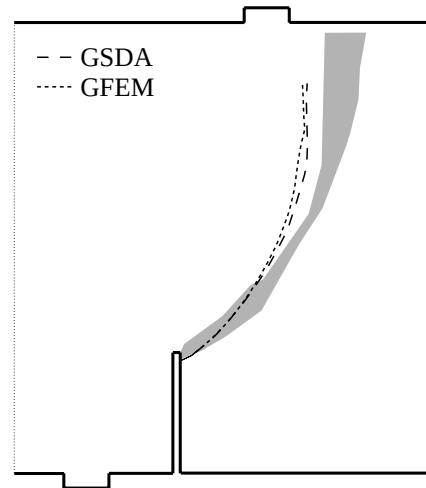
Figure 12. Four-point shear test: crack path.
