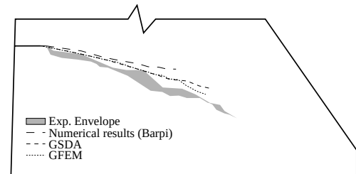
Figure 8. Prenotched gravity dam model: crack path.
