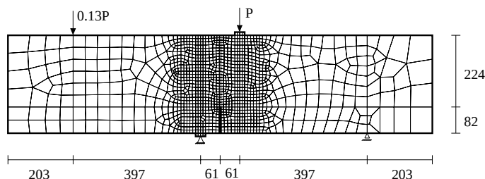
Figure 10. Four-point shear test: structural scheme (thickness 152 mm), including loading, boundary conditions and adopted mesh (all dimensions in mm).
