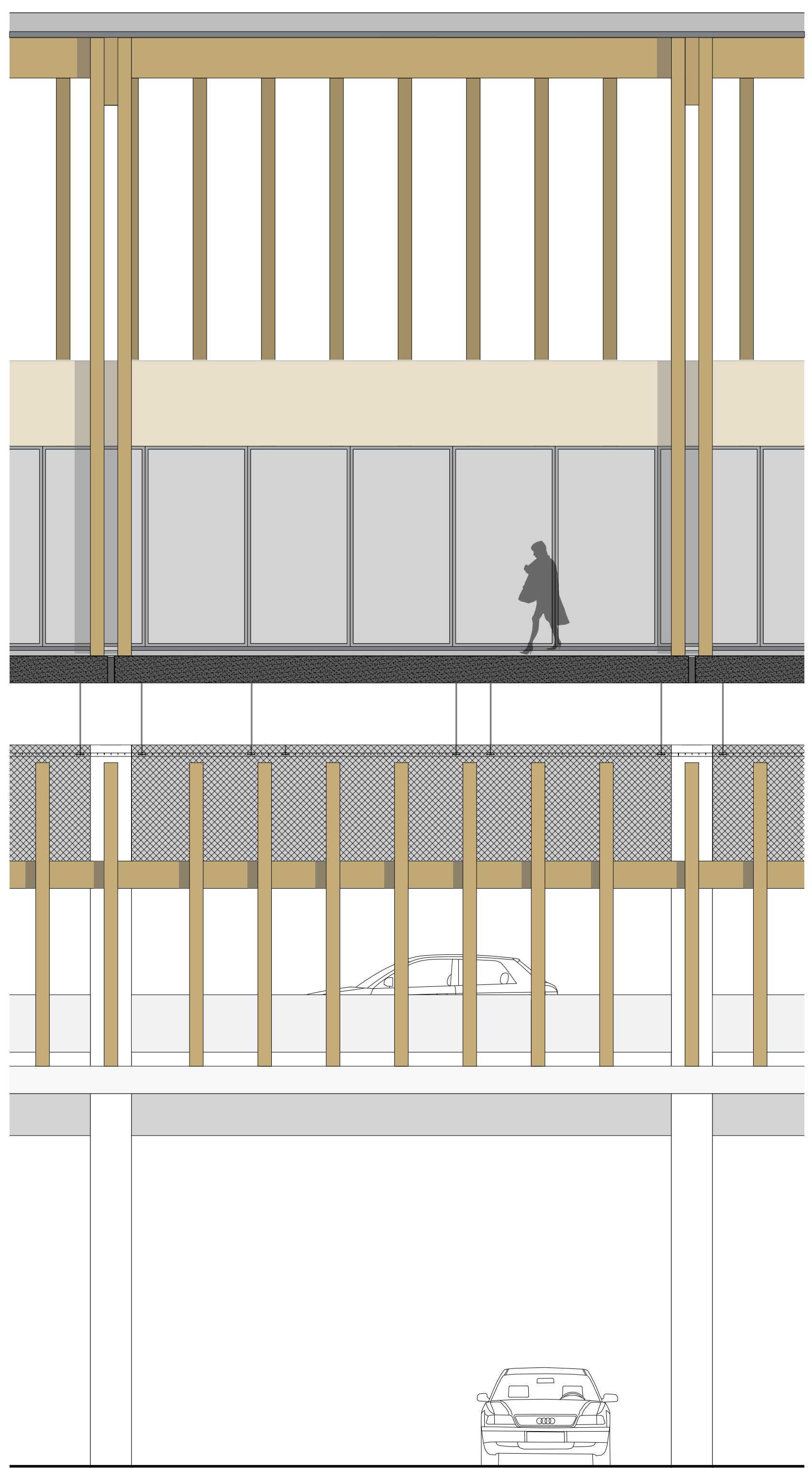
INSIDE FACADE FRAGMENT (S) 1:50
