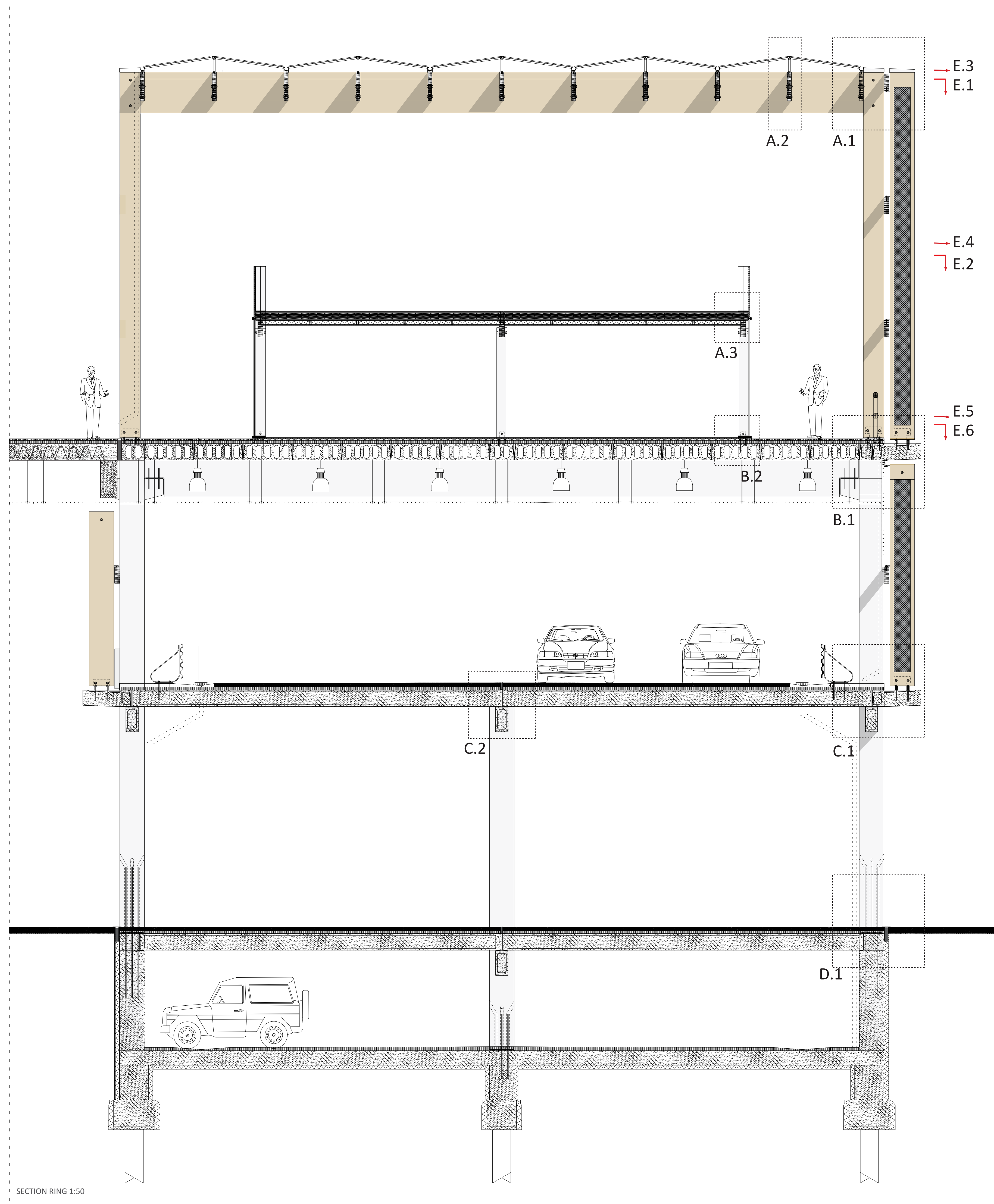
SECTION RING 1:50
