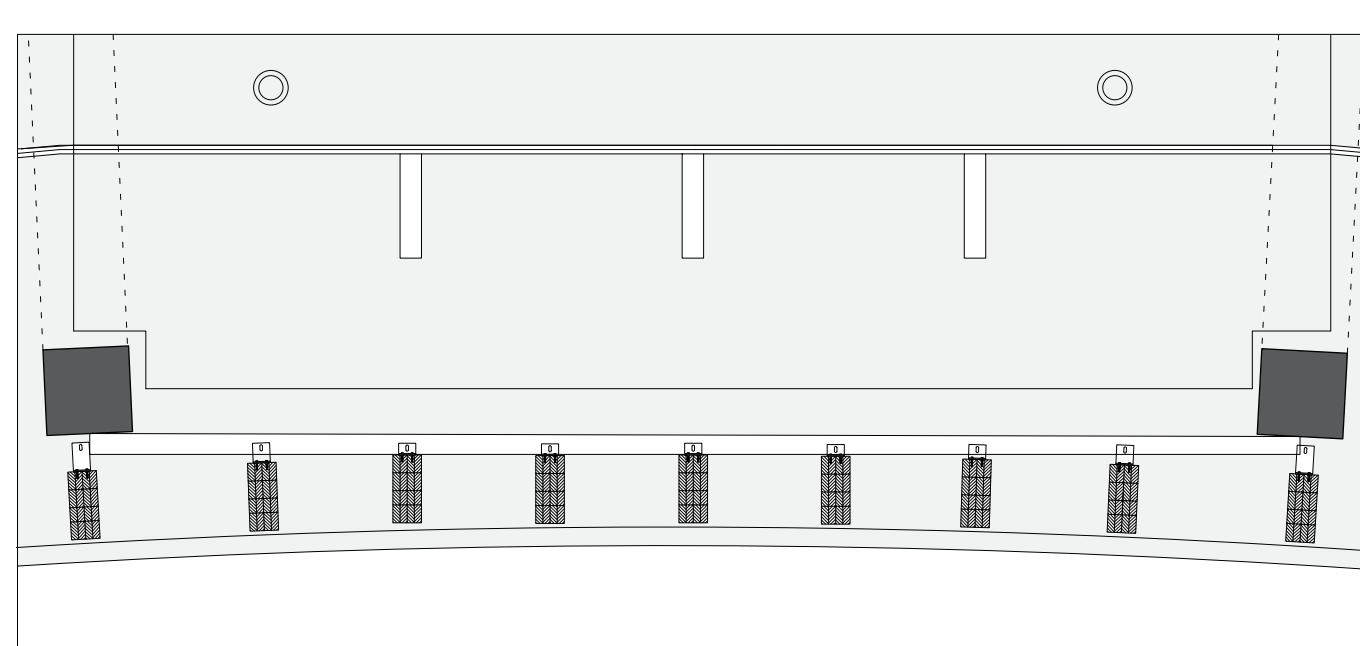
HORIZONTAL SECTION 2FLOOR (INSIDE)
