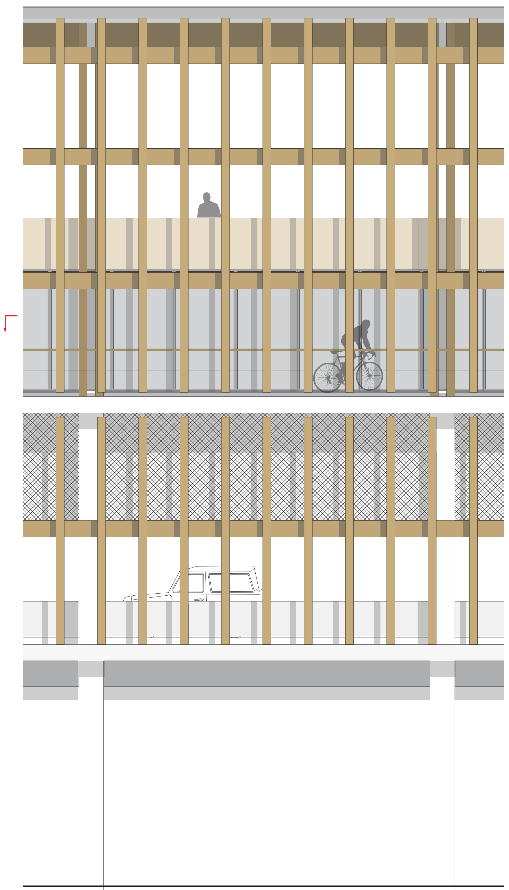
OUTSIDE FACADE FRAGMENT (N) 1:50
