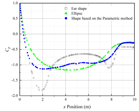
Fig.11 The mean pressure distribution along different SFT shapes
