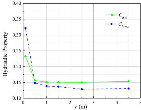
Fig.7 Hydraulic properties as a function of r
