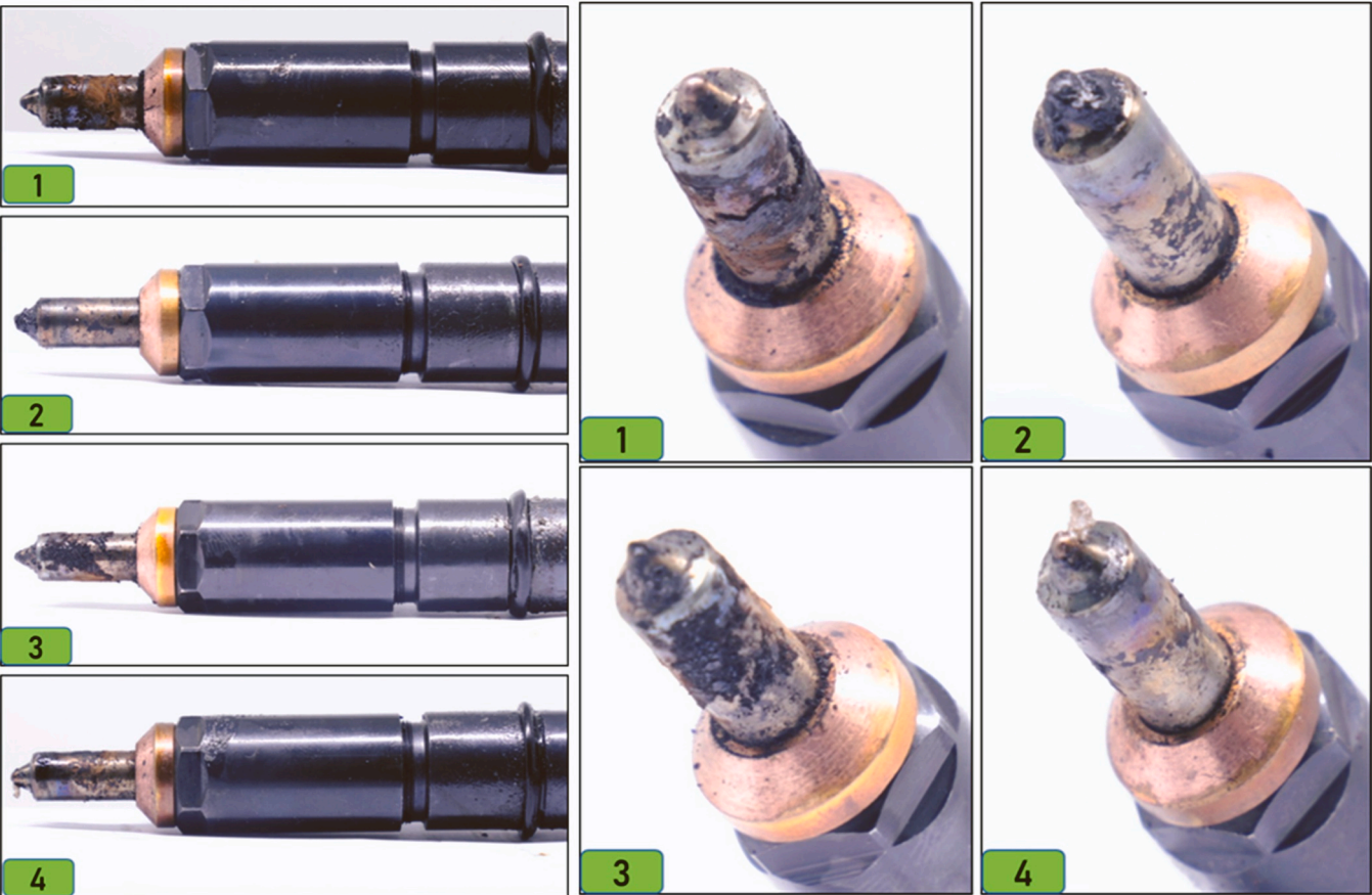
Fig. A23. The condition of injectors of the BPO engine after 500 operational hours.
