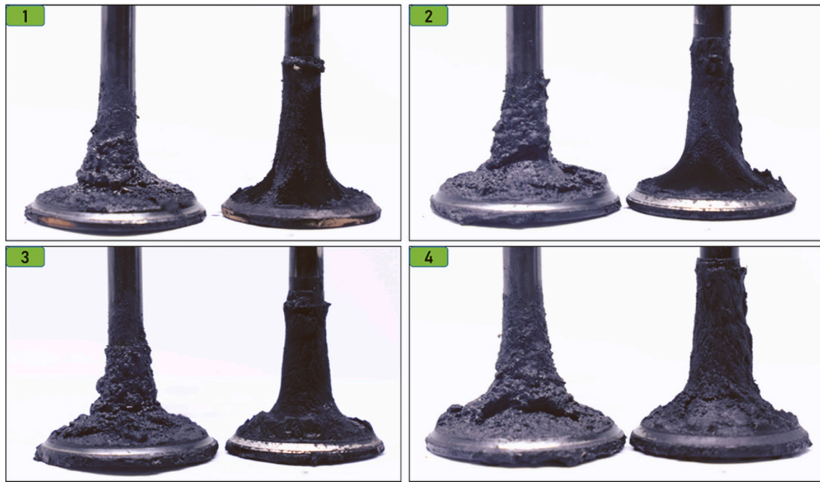
Fig. A17. The condition of intake valve and exhaust valve of the BPO engine after 500 operational hours.
