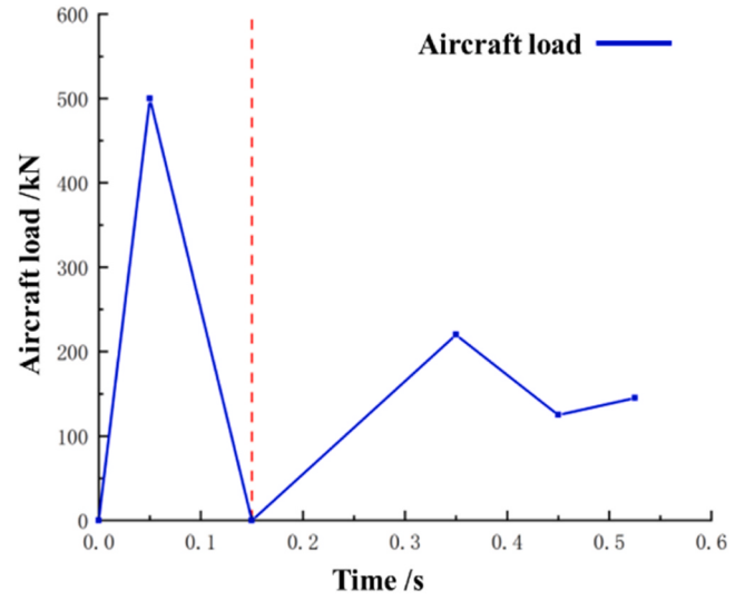
Fig. 5. Schematic of rough landing aircraft load.
