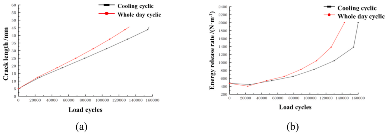
Fig. 11. Comparison between cracking features under the action of cooling cyclic and whole day's temperature range through (a) crack length, and (b) energy release rate.
