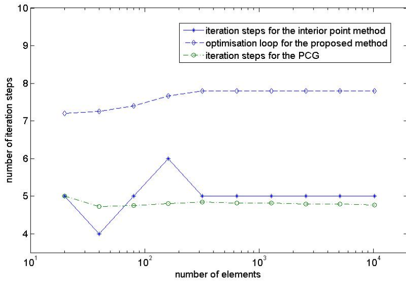
Figure 12: the Number of steps for entire optimization,interior point method and PCG
