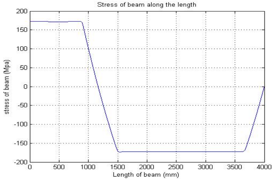
Figure 10: the normal stress on the top of the optimal beam
