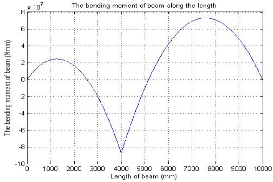
Figure 3: the bending moment in the optimal beam
