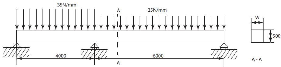
Figure 1: Two-span Continuous Beam
