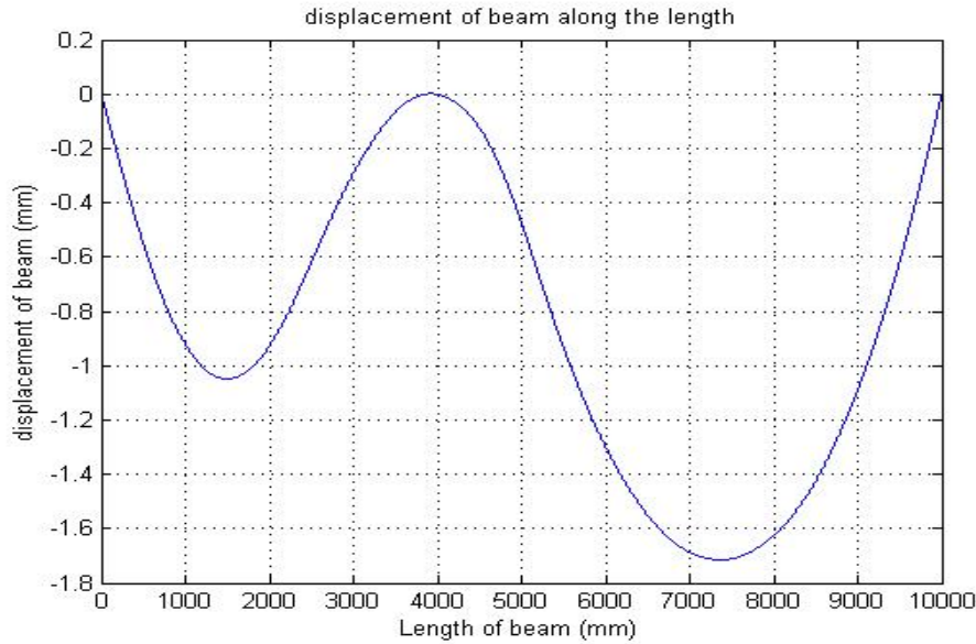
Figure 5: the displacement of the optimal beam
