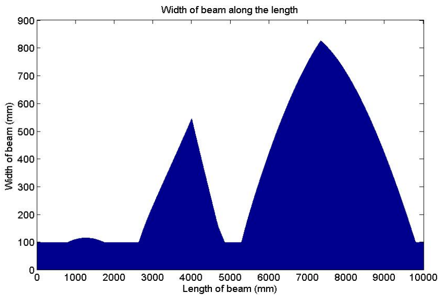
Figure 2: The width along the length of the optimal beam
