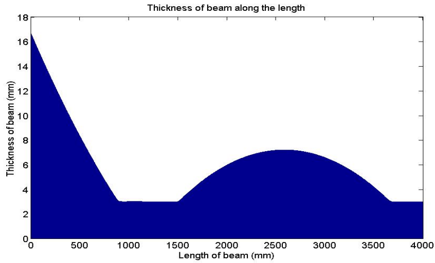
Figure 8: thickness along the length of the optimal beam
