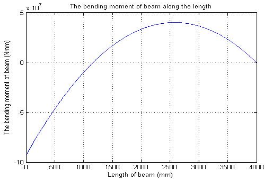
Figure 9: the bending moment in the optimal beam
