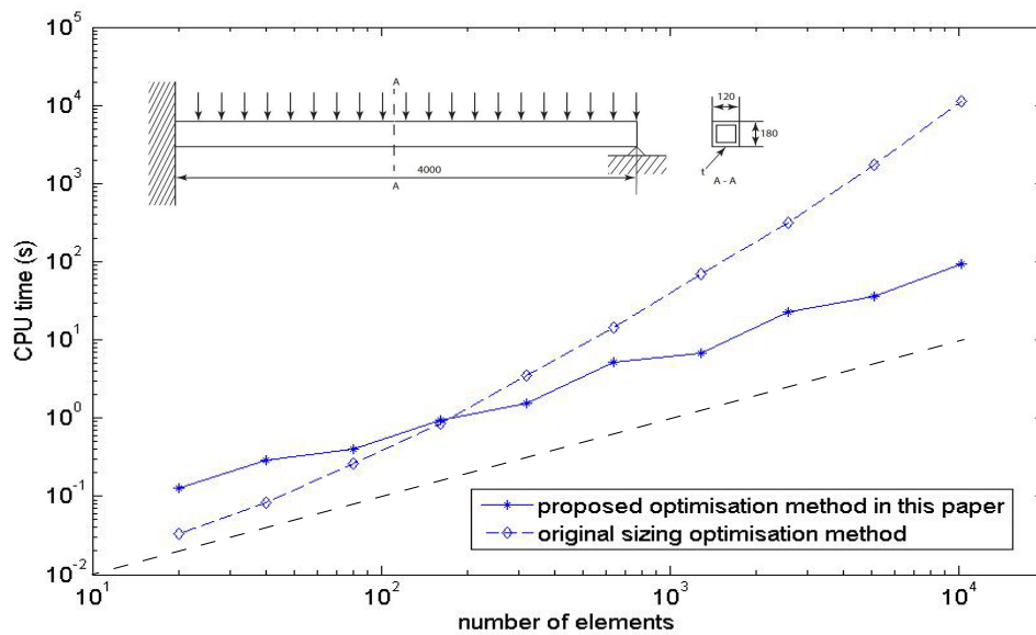
Figure 13: the log-log form of the CPU time vs number of elements for the optimization with original method and the proposed method
