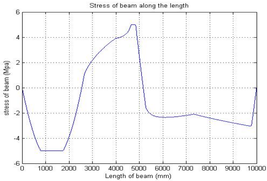
Figure 4: the normal stress on the top of the optimal beam
