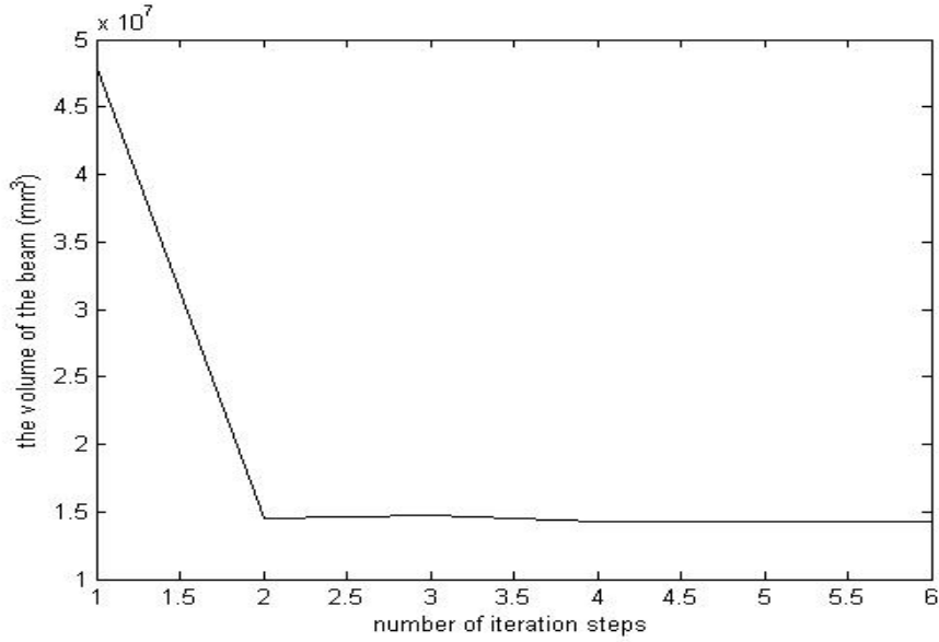
Figure 11: The volume of the beam in each iteration
