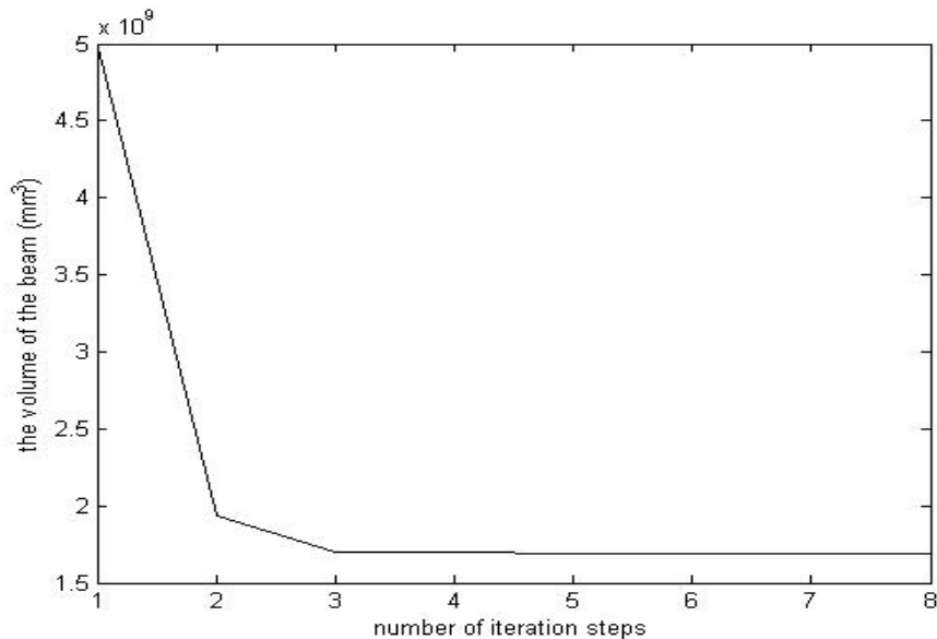
Figure 6: The volume of the beam in each iteration
