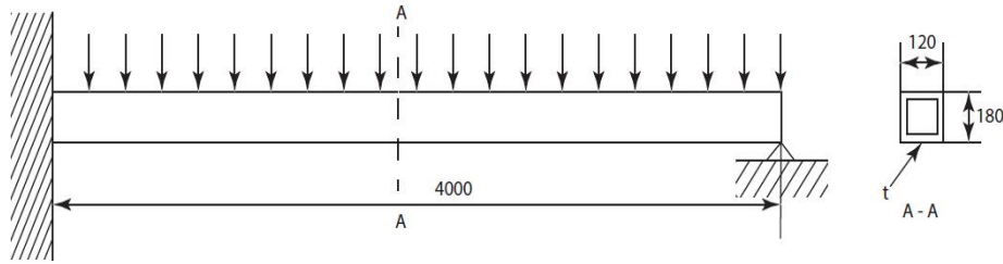
Figure 7: Hollow Beam Structure
