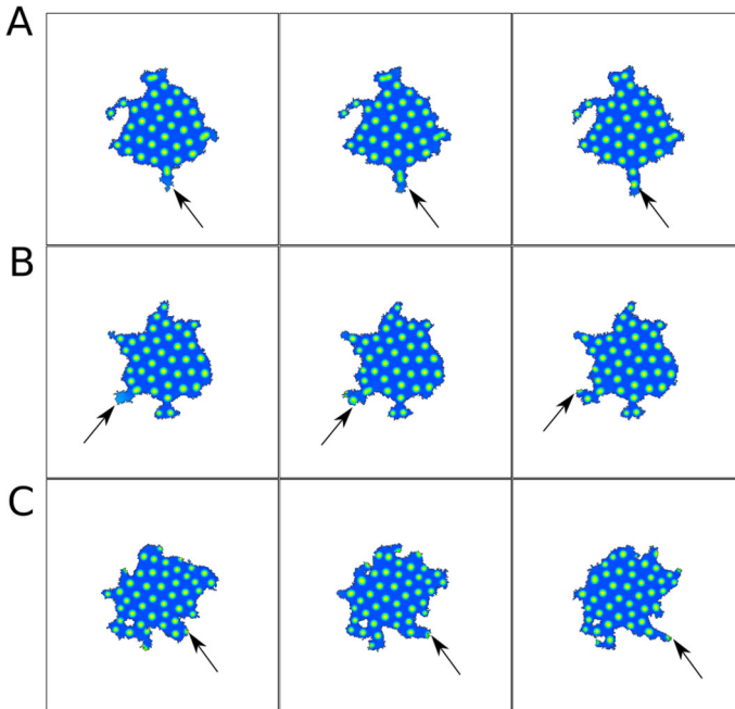
Fig. 21 Snapshots of 2D CPM simulation of the NC model. Visualized is \text{Rac}(u) that promotes protrusions ( H_0 = \pm\beta u ). Snapshots in A,B,C are 10,5,25 MCS apart respectively. Arrows indicate examples of interesting dynamics. a a spot breaks into two, b a new spot is created in a protrusion, c a spot leads a protrusion to form. Parameters are: \delta = 0.1 , \eta = 60 , k = 6 , \gamma = 120 , \theta = 18 , \alpha = 6 , and the rest from Table 4 (NC). CPM Parameters are: a = 10000 , \lambda_a = 0.02 , p = 1000 , \lambda_p = 0.04 , J = 40 , r = 3 , \xi(r) = 18 , \beta = 200 , T = 20 . Movie link https://imgur.com/yUUEgQD
