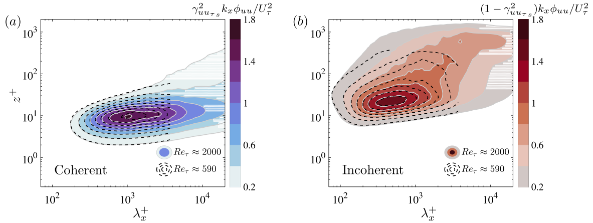
Fig. 4. Reynolds number comparison of wall-coherent and wall-incoherent portions of the pre-multiplied energy spectrograms (levels: 0.2:0.2:1.6). (a) Coherent portion, \gamma_{uu\tau}^2 k_x \phi_{uu} / U_\tau^2 . (b) Incoherent portion, (1 - \gamma_{uu\tau}^2) k_x \phi_{uu} / U_\tau^2 . Dashed line contours, Re_\tau \approx 590 ; filled contours, Re_\tau \approx 2000 . Spatial data are used to computed these correlation spectra.
