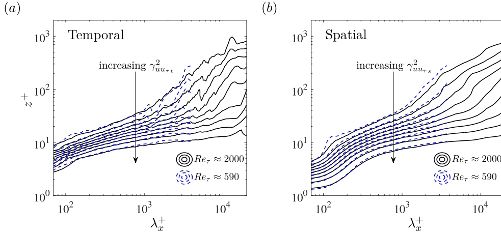
Fig. 3. Reynolds number comparison of coherence spectrograms (levels: 0.1:0.1:0.9). (a) Temporal spectrograms \gamma_{uu\tau_t}^2 . (b) Spatial spectrograms \gamma_{uu\tau_s}^2 . Dashed lines, Re_\tau \approx 590 ; solid lines, Re_\tau \approx 2000 .
