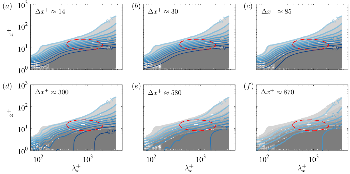
Fig. 8. Effect of streamwise distance between wall reference sensor and actuation points ( \Delta x ) on the spatial coherence spectrogram \gamma^2_{uu_x} at Re_\tau \approx 590 . The filled contours show the coherence spectrogram for \Delta x^+ = 0 (levels: 0.1:0.1:0.9), while the contour lines show coherence spectrograms for varying \Delta x^+ . Dashed lines show u -energy spectra contour level k_x^+ \phi_{uu}^+ = 1.8 and '+' markers show the peak in the energy spectrogram. (a) \Delta x^+ \approx 14 ; (b) \Delta x^+ \approx 30 ; (c) \Delta x^+ \approx 85 ; (d) \Delta x^+ \approx 300 ; (e) \Delta x^+ \approx 580 ; (f) \Delta x^+ \approx 870 .
