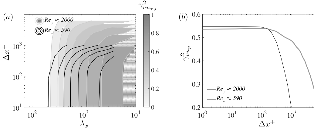
Fig. 9. (a) Reynolds number effect on the spatial coherence spectrogram at z^+ = 15 as a function of \lambda_x^+ and \Delta x^+ . Contour lines are associated with Re_\tau \approx 590 while filled contours correspond to Re_\tau \approx 2000 . Contour levels start from 0.1 in steps of 0.1. (b) Coherence magnitude at the near wall energy site, i.e. z^+ = 15 and \lambda_x^+ = 810 as a function of \Delta x^+ . Vertical dotted lines show \Delta x^+ = \delta^+ for Re_\tau \approx 590 and 2000 .
