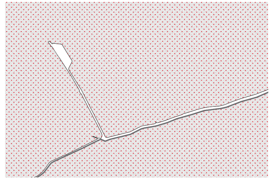
Extreme sea rise
