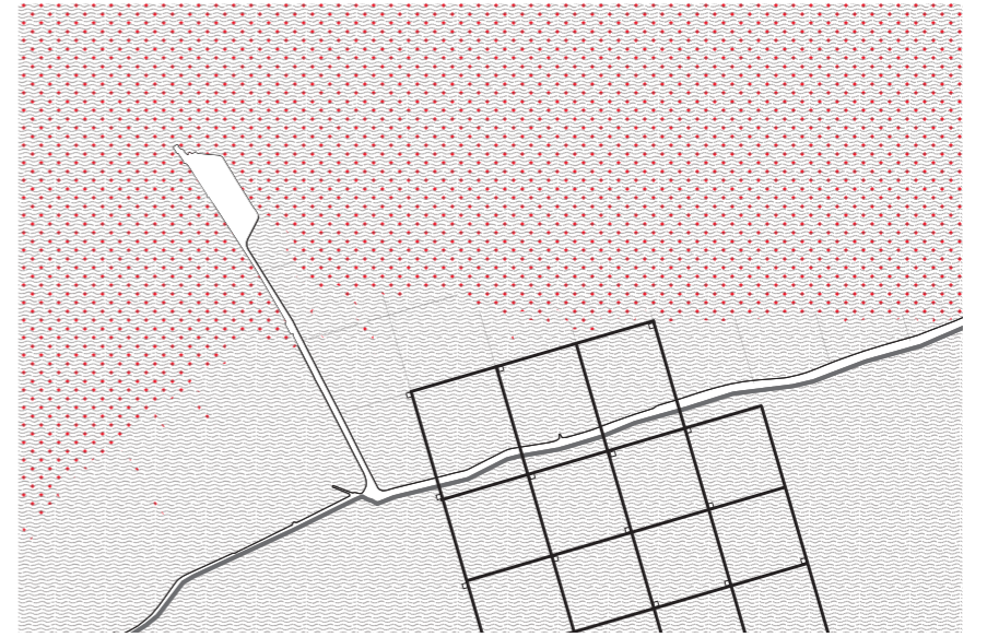
Expansion with sea level rise
