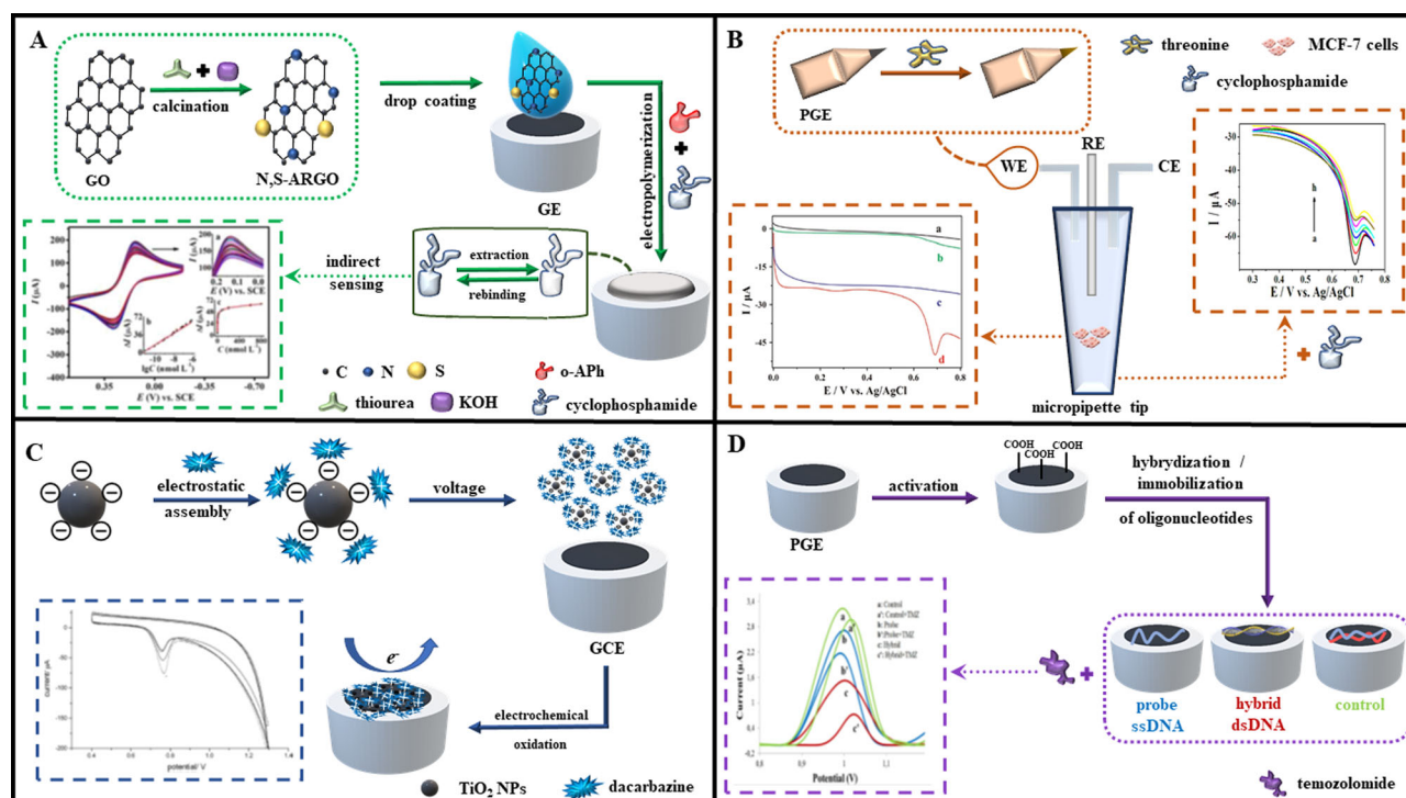
Figure 2. (A) The scheme showing the preparation of the sensor based on the graphite electrode (GE) containing N,S-ARGO and MIP with o -aminophenol ( o -APH) as a functional monomer developed for cyclophosphamide sensing. Voltammograms were reprinted from [51] with permission from Elsevier; (B) The schematic draw of the mini-electrochemical system constructed by integrating PGE modified with threonine as the working electrode and a micropipette tip having sealed ending as an electrochemical cell used for the investigation of the sensitivity of cyclophosphamide on the MCF-7 cells. Voltammograms were reprinted from [53] with permission from Elsevier; (C) The schematic representation of the biomolecular binding behavior of dacarbazine with DNA in the presence of the TiO 2 NPs. Voltammograms reprinted from [63] with permission from Elsevier; (D) The preparation of DNA biosensor based on anodically pretreated PGE developed for the investigation of the electrochemical interaction between methylated DNA sequences and temozolomide. The voltammetric signal differences enabled distinguishing ssDNA and dsDNA without using a label or tag. Voltammograms were reprinted from [66] with permission from Wiley.
