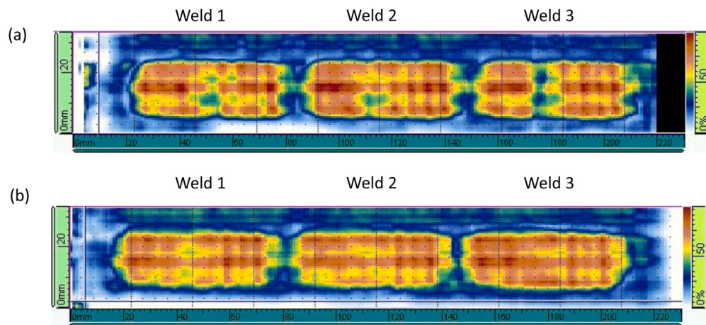
Fig. 4. NDI C-scan results: (a) Welds for specimen 1–3, with indications (<50% attenuation zones); (b) Welds for specimen 7–9, more consistent quality welds (all >50% attenuation). (For interpretation of the references to color in this figure legend, the reader is referred to the web version of this article.)
