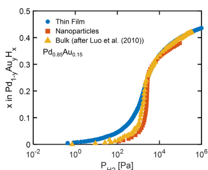
Figure 4. Comparison of the hydrogen solubility of a thin film ( T = 28\text{ }^{\circ}\text{C} ), a nanoparticle thin film ( T = 28\text{ }^{\circ}\text{C} ) and bulk material ( T = 30\text{ }^{\circ}\text{C} ) of \text{Pd}_{0.85}\text{Au}_{0.15} . The measurements were performed by stepwise increasing the hydrogen pressure. The bulk data are adapted from ref 22.
