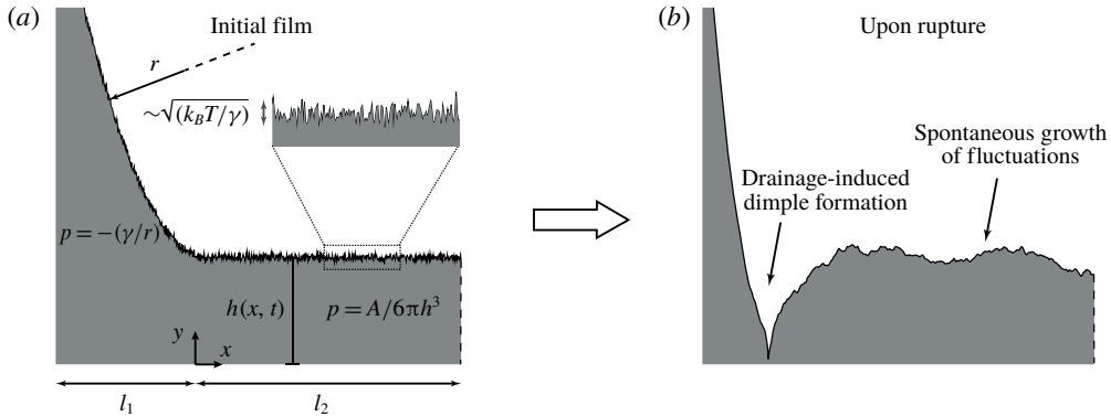
FIGURE 1. Schematic of a non-flat draining thin film subjected to thermal fluctuations, with the film thickness parameterized by h(x, t) . (a) The initial film shows a curved part extending from -l_1 \leq x < 0 with the pressure given by the Laplace pressure, p = -\gamma/r , with 1/r as the curvature imposed at the edge. This curved part is connected to a flat part extending from 0 \leq x \leq l_2 with the pressure given by the van der Waals component of the disjoining pressure, p = A/6\pi h^3 . Besides curvature-induced drainage, the film is also subjected to thermal fluctuations of the free interface, resulting in thickness variations of amplitude \sim \sqrt{k_B T/\gamma} . The dashed line at x = l_2 signifies the symmetry in the system. (b) Shape upon rupture, highlighting that film thinning stems from two competing mechanisms: (1) the formation of a localised dimple due to curvature-induced drainage and (2) the spontaneous growth of waves originating from thermal fluctuations.
