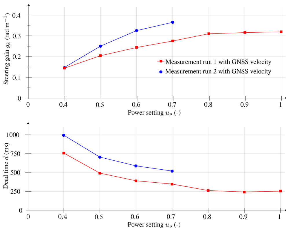
Figure 23. Comparison of the mean values of steering gain g_k and dead time d averaged over both tow directions as functions of the power setting u_p for the Vegas 2015 kite with a 10 m 2 wing surface area when performing the MLE with the GNSS velocity. Adapted from Elfert (2021).
