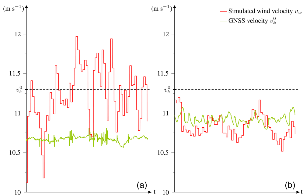
Figure 24. Representative cut-outs of the simulated wind and GNSS velocity data during a period of equal length in the first (a) and second (b) measurement run. Tow speed set to v_b^0 = 11.3 m s -1 . Adapted from Elfert (2021).
