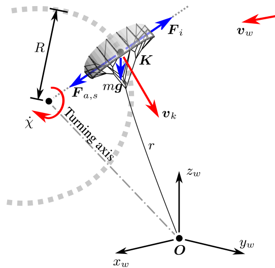
Figure 5. Kite performing a left turn with a turning radius R tethered to a fixed point O on the ground.
