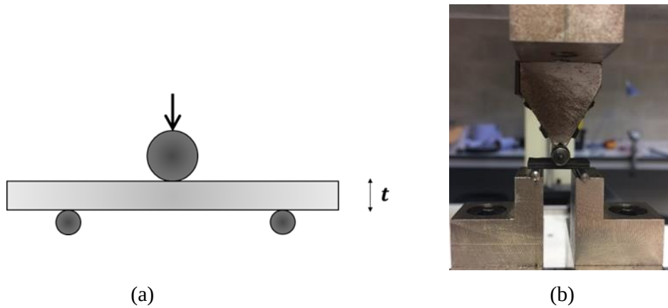
Fig. 3. ILSS test details: (a) Schematic representation and (b) ILSS test setup.
