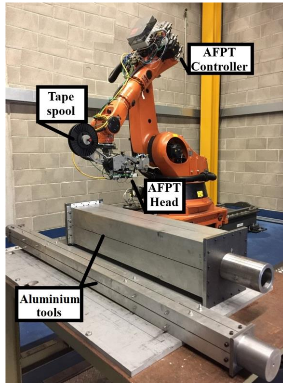
Fig. 1. LATP setup and aluminium tools.
