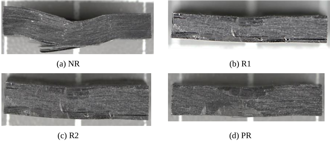
Fig. 9. Influence of laser repress on the interlaminar shear failure of UD [0^\circ]_{16} laminates.
