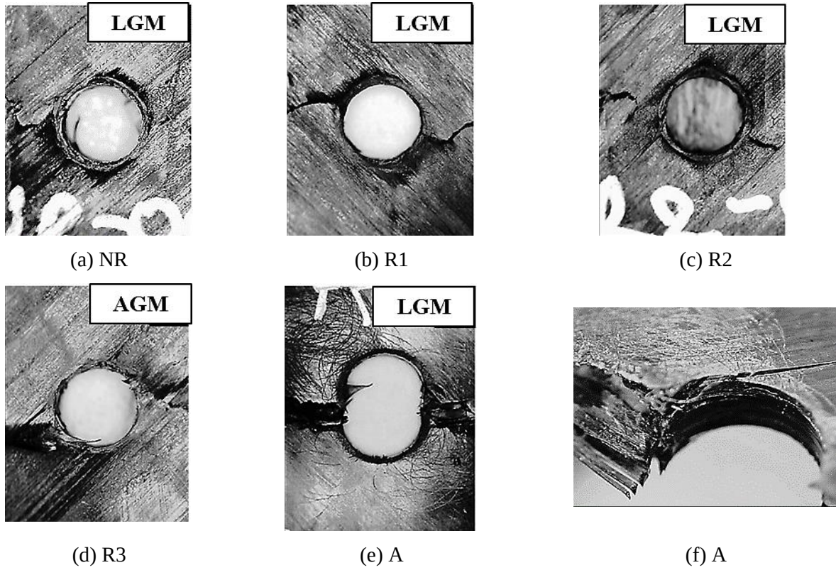
Fig. 12. Details of failure modes from the top view of the hole areas for the OHC specimens, both lateral (LGM) and angled (AGM) failure types: (a) no repass, (b) single repass (c) double repass, (d) tool-side repass, (e) autoclave-1 and (f) autoclave side view.
