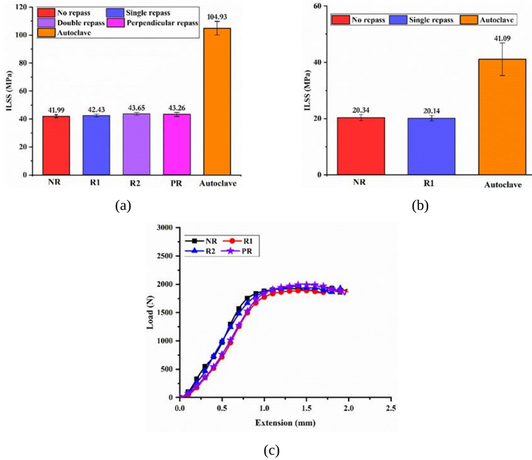
Fig. 8. Influence of repress on the ILSS: a. UD [0^\circ]_{16} , (b) Angle-ply [\pm 45^\circ]_{4s} and (c) Typical load-extension response.
