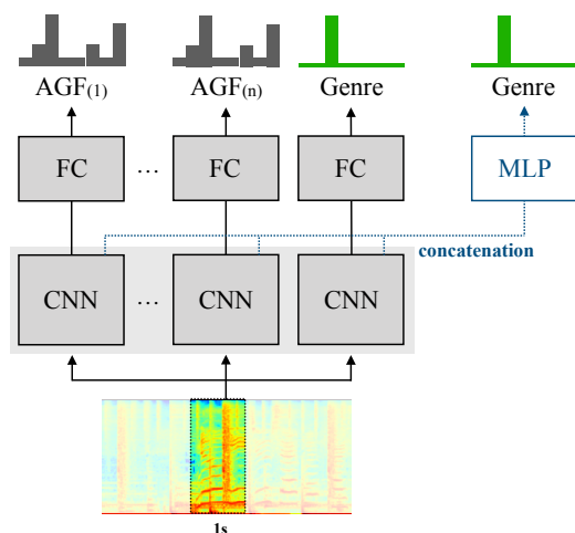
Figure 2: Illustration for the transfer learning scenario. Dotted lines indicate the setup for the multilayer perceptron for performing final genre classification.
