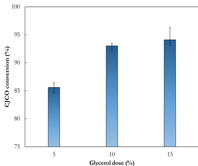
Fig. 2 Effect of glycerol dosage for CaO activation. Reaction temperature: 65 °C, time: 420 min, CaO amount: 15 wt%, methanol-to-CJCO molar ratio: 9:1, stirring intensity: 350 rpm
