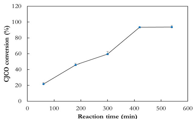
Fig. 4 Effect of reaction time on CJCO conversion. Reaction temperature: 65 °C, CaO amount: 15 wt%, glycerol dosage: 10 wt%, methanol-to-CJCO molar ratio: 9:1, stirring intensity: 350 rpm
