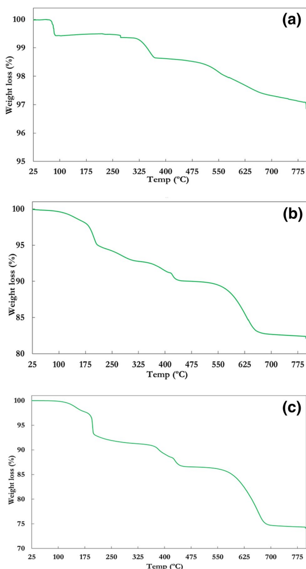
Fig. 8 Thermal analysis for CaO and glycerol-enriched CaO. a Mussel shells derived CaO-fresh, b glycerol-enriched CaO-fresh, c glycerol-enriched CaO-collected
