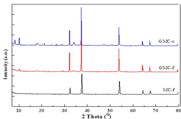
Fig. 7 XRD patterns for CaO and glycerol-enriched CaO. MC-f muschel shells derived CaO-fresh, GMC-f glycerol-enriched CaO-fresh, GMC-c glycerol-enriched CaO-collected
