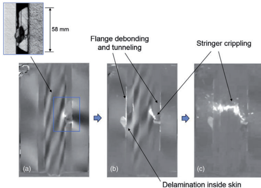
Figure 14. Infrared images illustrating sequence of collapse (SSCS-4). (a) Delamination reaches critical size, (b) unstable tunneling, and (c) stringer crippling.
