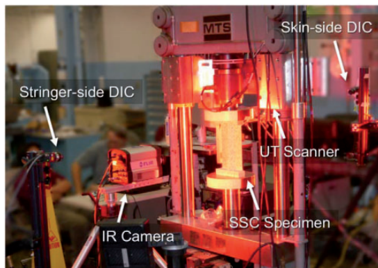
Figure 8. SSC specimen, load frame, and test instrumentation.
