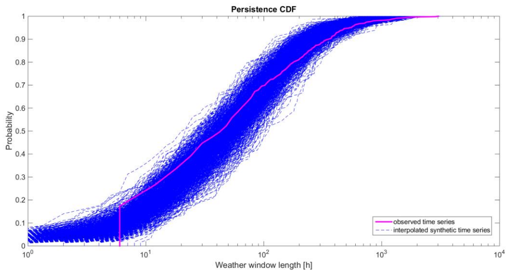
7 Figure 18: Comparison between CDF of the observed persistence and CDF of persistence for 1000 interpolated 8 synthetic time series (1h).
