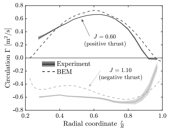
Fig. 12 Comparison of the propeller blade circulation distribution between BEM and experimental data for two different thrust settings.
