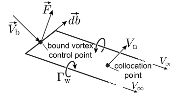
Fig. 11 Close-up of a single horseshoe vortex with the collocation and bound vortex control point.
