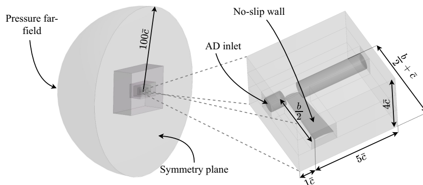
Fig. 18 Numerical domain and boundary conditions for the RANS simulations.
