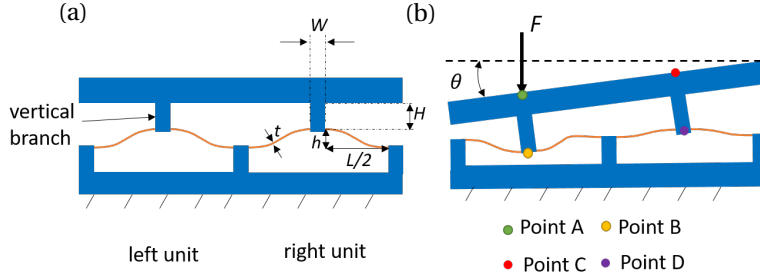
Figure A.1: The unit cell. (a) Structural geometry of the unit. b represents the out-of-plane dimension. (b) Illustration of the deformation of the unit when a point load applied at Point A.
