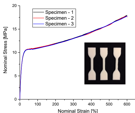
Figure D.3: Stress-strain curves for the material are obtained by standard tensile tests.
