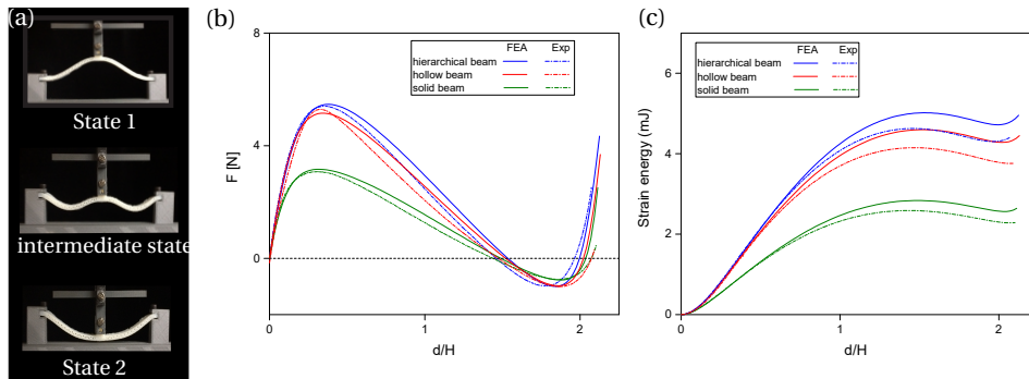
Figure 4.3: Snap-through behavior of unit cells. (a) Snapshots of a hierarchical beam during the un-axial loading. (b) The measured and simulated force-displacement curves of the hierarchical, hollow and solid beams. (c) Evolution of the unit cell's strain energy during the uniaxial loading.
