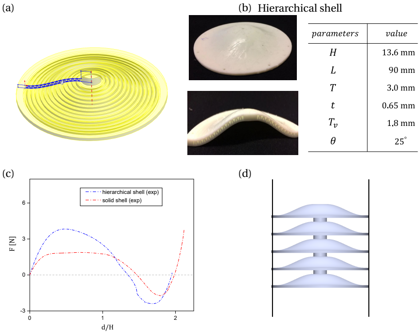
Figure 4.10: The lattice-based shell structures. (a) The shell structure is developed by a revolution of the hierarchical beam profile (in blue) along the axis of rotation (red dashed line). (b) A real demonstration of the shell and its cross section. Geometric parameters are depicted. (c) The experimentally characterized force-displacement responses of the hierarchical and the solid shell. (d) An illustration of a serial arrangement of hierarchical shells for energy absorption.
