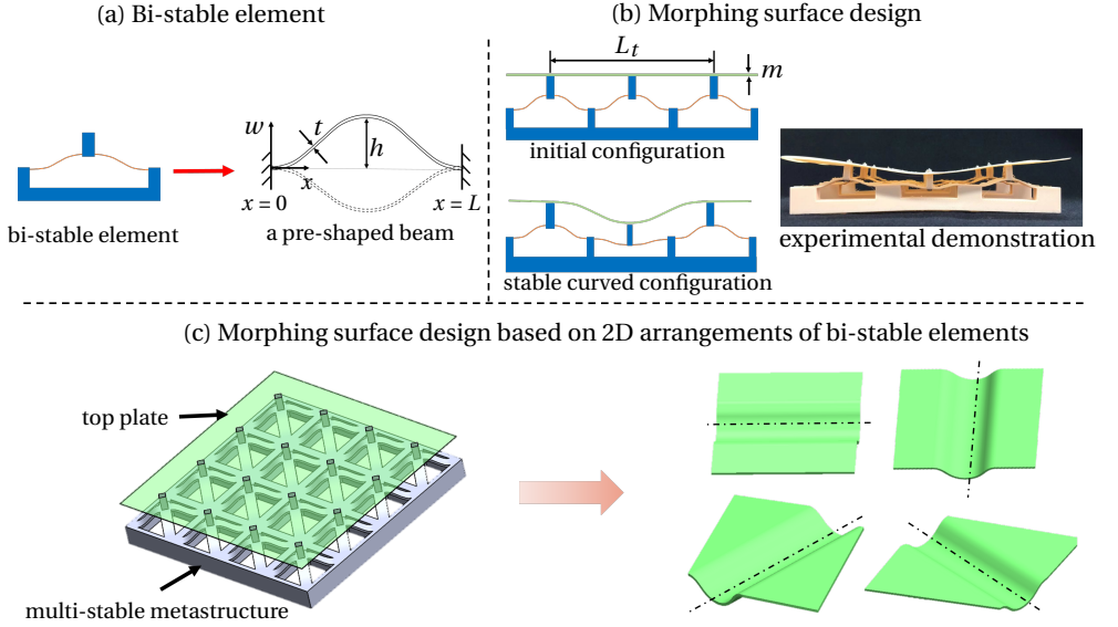
Figure 5.1: Schematic diagram of the proposed multi-stable surface design. (a) For each bi-stable element, a pre-shaped curved beam is able to snap into a second stable state (illustrated by curved dashed lines). (b) Morphing surface design. A thin compliant plate is connected with a multi-stable metastructure here composed of three bi-stable elements. When the center element snaps, the plate can stabilize at the curved configuration. Picture on the right shows an experimental demonstration of the stable curved configuration. (c) Morphing surface design based on 2D arrangements of bi-stable elements. When multiple bi-stable elements snap, the curved stable configurations can be oriented in different directions, as depicted by the dot lines.
