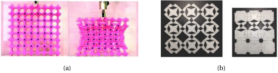
Figure 1.1: Examples of flexible metastructure design. (a) A flexible metastructure that can achieve configuration transformations under compression [10]. (b) A reconfigurable metastructure is based on compliant hinges with rotational degrees of freedom [11]. Panel (a) is adapted with permission from Ref. [10], John Wiley & Sons, Inc. Panel (b) is adapted with permission from Ref. [11], John Wiley & Sons, Inc.
