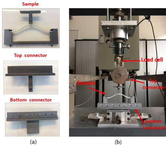
Figure C.2: The experimental setup of loading tests. (a) The sample, top and bottom connector. (b) The uniaxial loading test.
