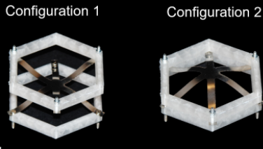
(c) 3D unit cell – two level configurations
