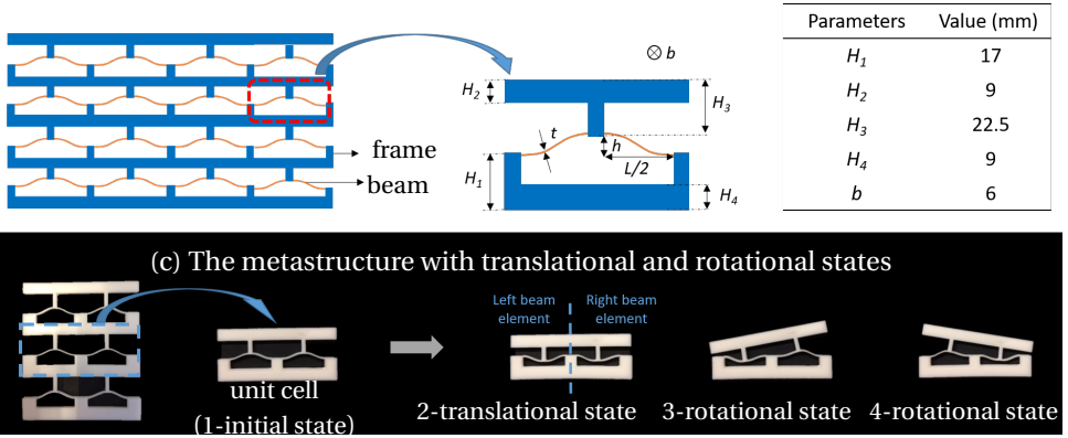
Figure 2.1: A demonstration of multi-stable structures with translational and rotational stable states. (a) A schematic for the proposed multi-stable metastructure. The structure is designed by serially stacking curved beams with thick frames. (b) Geometric parameters of the beam element are depicted. The out-of-plane dimension is denoted as b . (c) Each unit cell ( h = 5\text{mm} , t = 0.8\text{mm} and L = 28\text{mm} ) possesses four stable states such that it can snap into the translational state or the rotational states.
