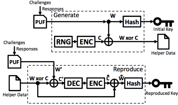
Figure 2.2: Generation and reproduction procedures of fuzzy extractor on PUF [43].
