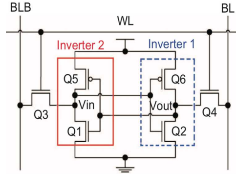
Figure 2.3: A 6-T CMOS SRAM cell [37].
