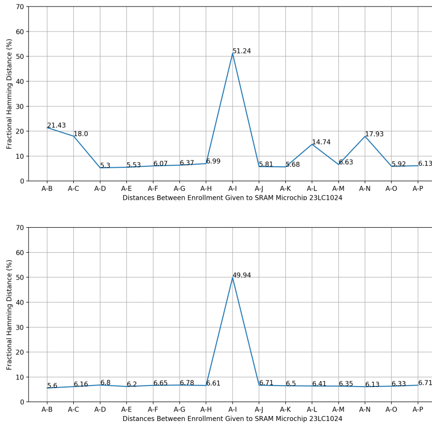
Figure 4.10: Time interval testing results on SRAM Microchip 23LC1024. The top figure is the testing result on stable bits generated using neighbor analysis, while the bottom one is tested on stable bits generated using data remanence approach. Index A on x-axis refers to enrollment on day 1, B on day 2, etc. Index A-B refers to fractional hamming distance between enrollment on day 1 and day 2.
