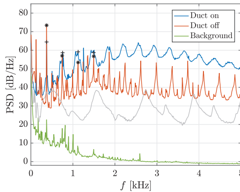
Figure 7. Averaged spectrum level over the microphones for the propeller at 85% of the maximum power corresponding to a propeller speed of 7500 r/min. The stars and crosses indicate the BPF and its first three multiples for the isolated and ducted propeller, respectively. As a comparison the ducted omni-directional sound source is shown in gray.
