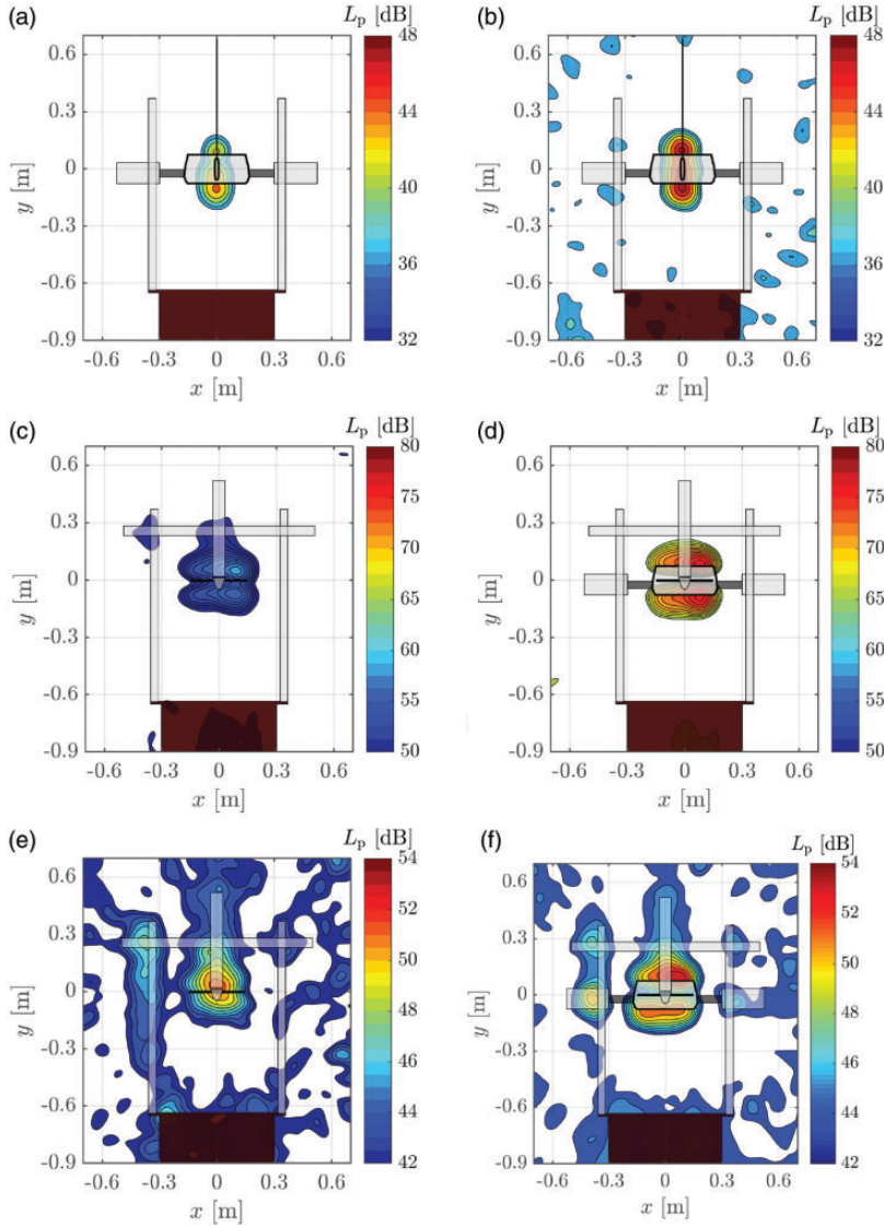
Figure 11. Beamforming of the omni-directional source for frequencies of the peaks and valleys observed in Figure 5, and for the isolated and ducted propeller with and without incoming inflow. (a) Valleys. (b) Peaks. (c) Isolated propeller, with no incoming airflow. (d) Ducted propeller, with no incoming airflow. (e) Isolated propeller, with a constant incoming airflow. (f) Ducted propeller, with a constant incoming airflow.
