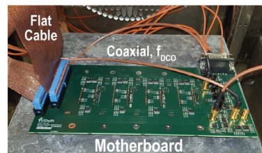
Figure 3.4.S1: The frequency-reference measurement setup (top) consists of a motherboard carrying 4 samples. This is placed in an oven, and the samples are controlled by an FPGA. The PC (via a DAQ card) is only used to control the measurement setup.
