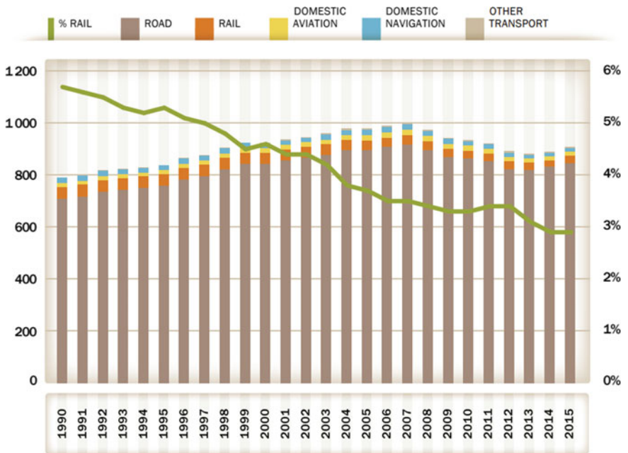
Fig. 1.3 Transport sector CO 2 emissions by mode, 1990–2015 (million t CO 2 —left, rail share over total—right. Note: Electricity and heat production related emissions are reallocated to the end-use sectors.) [2]
