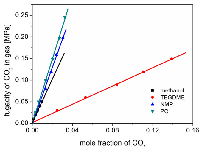
Figure 2. (Colour online) Solubility of CO 2 in methanol at 248 K, and in TEGDME, NMP, and PC at 298 K.
