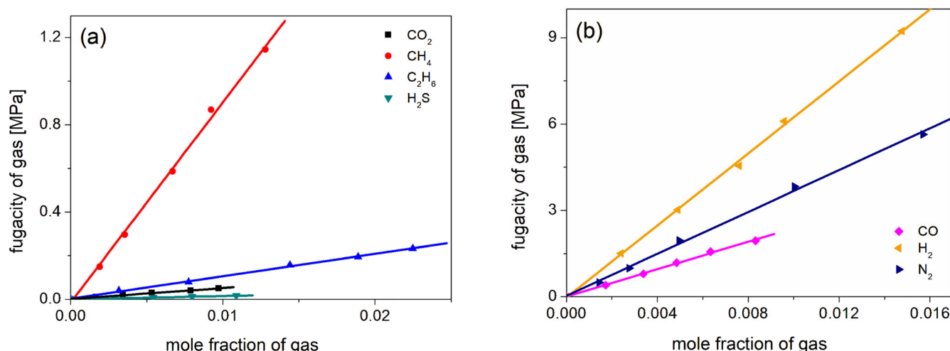
Figure 3. (Colour online) (a) Solubility of CO 2 , CH 4 , C 2 H 6 , and H 2 S in methanol at 248 K. (b) Solubility of CO, H 2 , and N 2 in methanol at 248 K.
