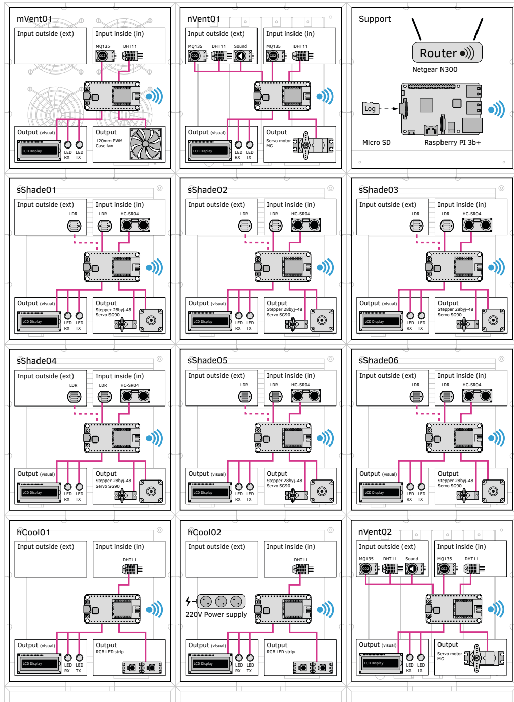
FIG. 5.5 Technical equipment of the prototype
