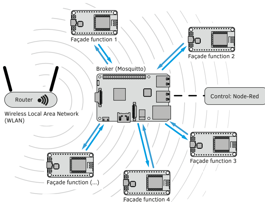
FIG. 5.6 Organization of the MQTT communication system derived from Joncas (MQTT and CoAP, IoT Protocols | The Eclipse Foundation, https://www.eclipse.org/community/eclipse_newsletter/2014/february/article2.php , (accessed November 11, 2019)
