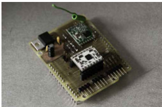
C SMART RFDUINO
