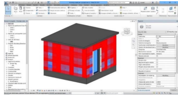
Figure 7: BIM based thermography related to the measured temperatures.
