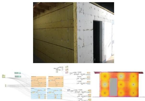
Figure 6: Test house before the installation of the finishing layers when it is possible to see the two target insulation materials, VPL model, and simulation of the spread radius of the temperature variation.
