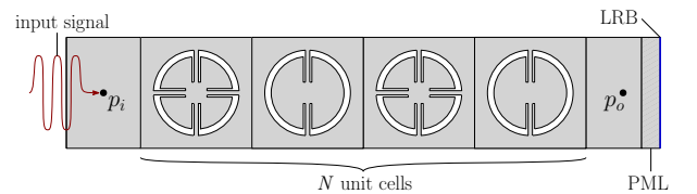
FIGURE 8. ARRAY OF N DIFFERENT UNIT CELLS USED FOR TRANSMISSION ANALYSIS.
