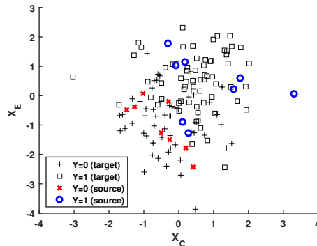
Figure 3: An example of synthetic classification data.
