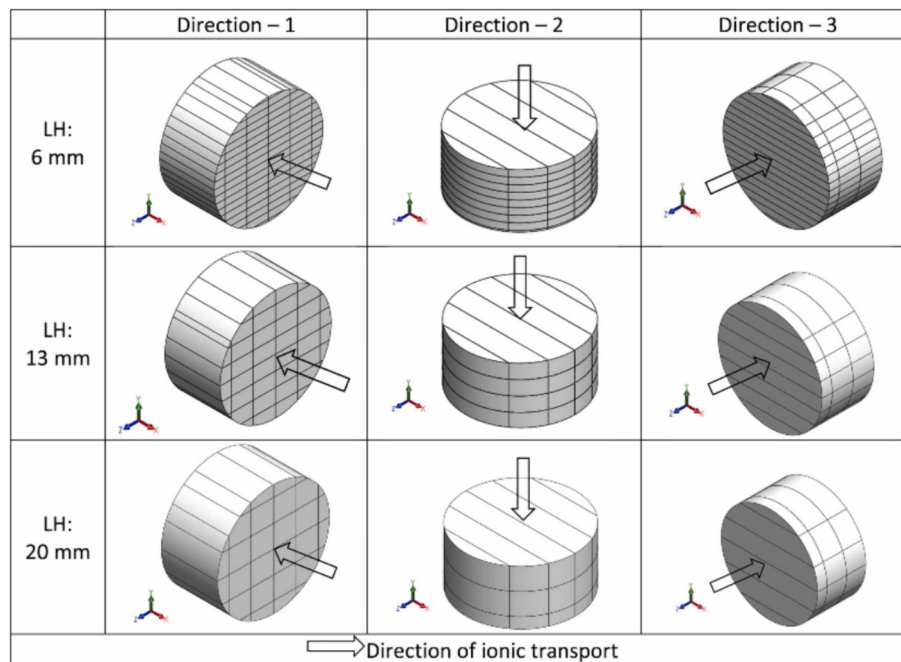
Fig. 9. Schematic illustration of ionic transport pathways in three orthogonal directions for specimens printed with different layer heights. The lighter shade represents the layers, while the darker shade indicates the interlayer region (taken from [86]).
