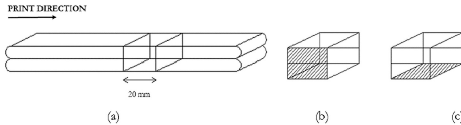
Fig. 5. Schematic depiction of the water exposure surfaces: (a) the original printed sample, (b) the 'front' water exposure surface, and (c) the 'bottom' water exposure surface (taken from [76]).
