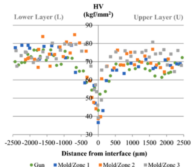
Fig. 4. Hardness value (HV) as a function of the distance from the interlayer measured on two-layered samples with a 24-hour time gap. Measurements were performed on a sample manually printed using a caulking gun ("Gun") and on three zones of a specimen printed with the caulking gun and compacted inside a mold ("Mold") (taken from [55]).
