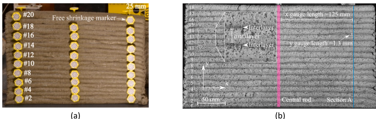
Fig. 10. Early-age shrinkage assessment in 3D printed wall element using (a) embedded markers and (b) chalk paint-based speckle pattern (taken from [103]).
