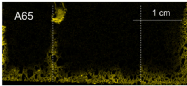
Fig. 11. Micro XRF chlorine map for sample exposed to chloride solution. Chloride penetration happened from the bottom surface and the interlayers indicated by dashed lines. Yellow colour indicates chloride ions and the intensity of the colour is proportional to the quantity of chloride ions (taken from [59]). (For interpretation of the references to colour in this figure legend, the reader is referred to the web version of this article.)
