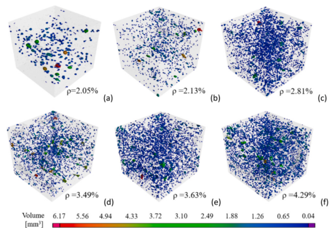
Fig. 12. Porosity visualization of 3DPC after exposed to (a) room temperature, (b) 200 °C, (c) 400 °C, (d) 600 °C, (e) 800 °C, and (f) 1000 °C [taken from [122]].
