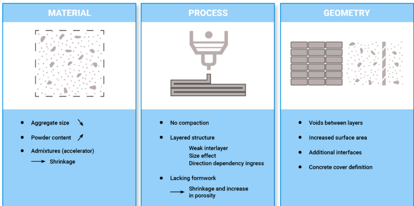
Fig. 1. Material-related, process-related and geometrical issues in 3DPC.
