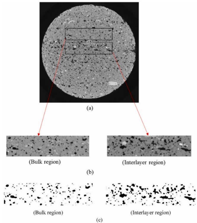
Fig. 3. Study of the porosity in the bulk and interlayer region by micro-CT: (a) slice from the 3D tomographic reconstruction of a cylindric sample, (b) details of the bulk and interlayer region, and (c) details of the porosity in the bulk and interlayer region (taken from [20]).
