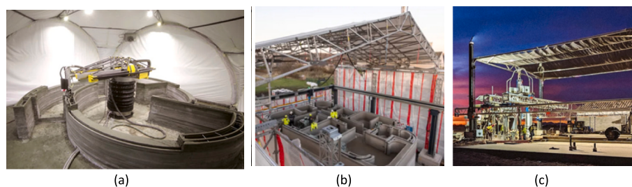
Fig. 14. On-site control and/or mitigation of environmental conditions during printing via a) complete enclosure [138], b) partial enclosure [139] or c) roof cover only [140].
