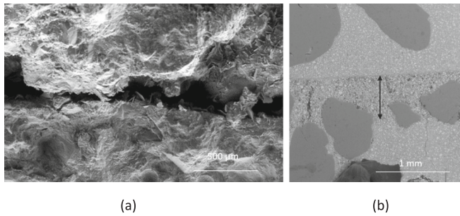
Fig. 2. Air inclusion (a) and drying (b) in the interlayer region as observed by SEM (taken from [32,36]).
