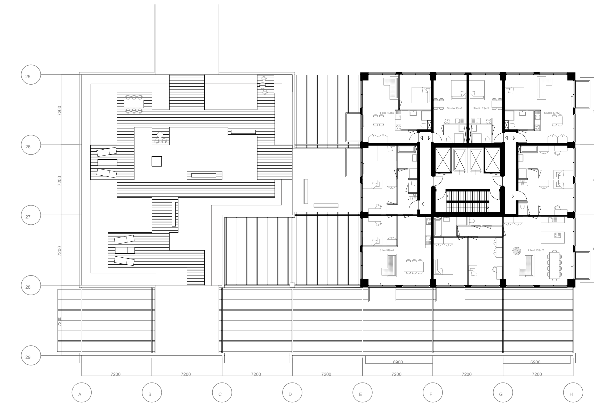
HOUSING FLOORPLAN
