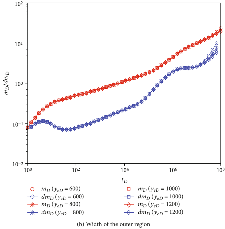
FIGURE 8: The effect of size of the outer region on pressure and derivative curves.
