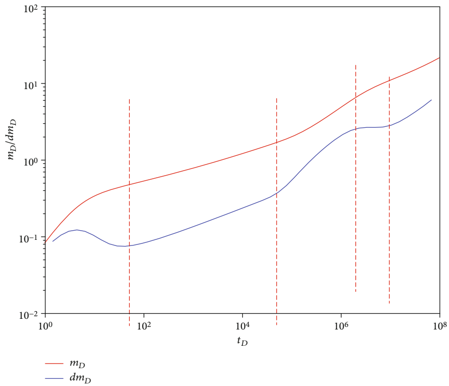
FIGURE 4: Typical curves of multifractured horizontal well in stress-sensitive SGR formation.
