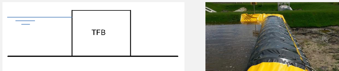
Figure 1 Schematic cross section of a Temporary Flood Barrier (left) and an example TFB (right) (source: www.tubebARRIER.com )
