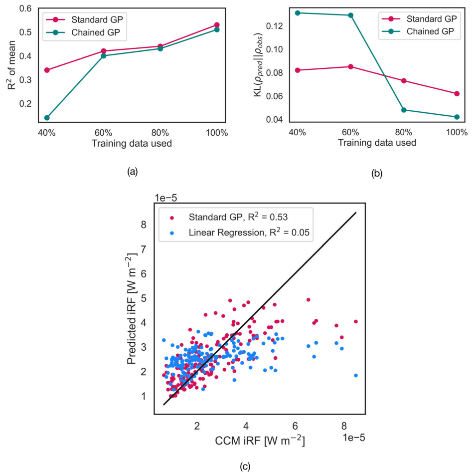
Fig. 4 | Convergence study of GP models and comparison with linear regression models. The complete dataset ( d ) is split into training data ( y ), which never exceeds 80% d , and test data ( y_* ). y_* is fixed at 20% d . We analyse if the standard GP (in crimson red) and chained GP (in teal) models perform better by gradually increasing the amount of training data for four scenarios: 40%, 60%, 80%, and 100% of y and testing them on y_* . a Convergence of R^2 of the mean predictions on the test data increases as more training data is used. b The statistical distance between the predictive distribution and the test data distribution shrinks in terms of KL divergence as more training data is used. c We compare the mean predictions of the linear regression model (in bright blue) against test data with (T, \phi, T \cdot \phi) as the feature basis. The mean predictions from the standard GP model (in crimson red) are overlaid as a reference, and the R^2 values are included in the legend.
