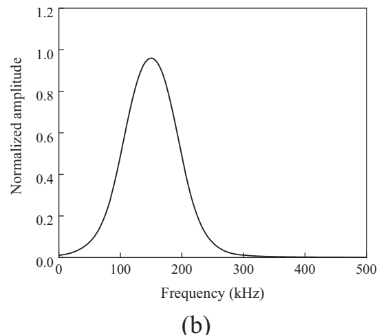
Fig. 9. The waveform used to generate signals: (a) time-domain and (b) frequency domain.
