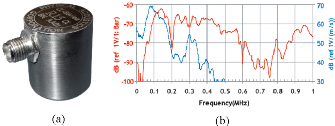
Fig. 4. (a) R15 \alpha AE sensor; (b) Frequency sensitivity spectrum of the R15 \alpha AE sensor.
