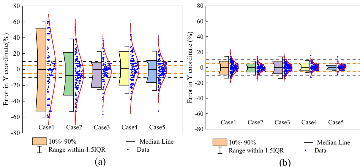
Fig. 26. Error distribution of all cases, limitation at \pm 10\% (black) and \pm 5\% (orange): (a) using the TOA method; (b) using ANN-based method. (For interpretation of the references to color in this figure legend, the reader is referred to the web version of this article.)
