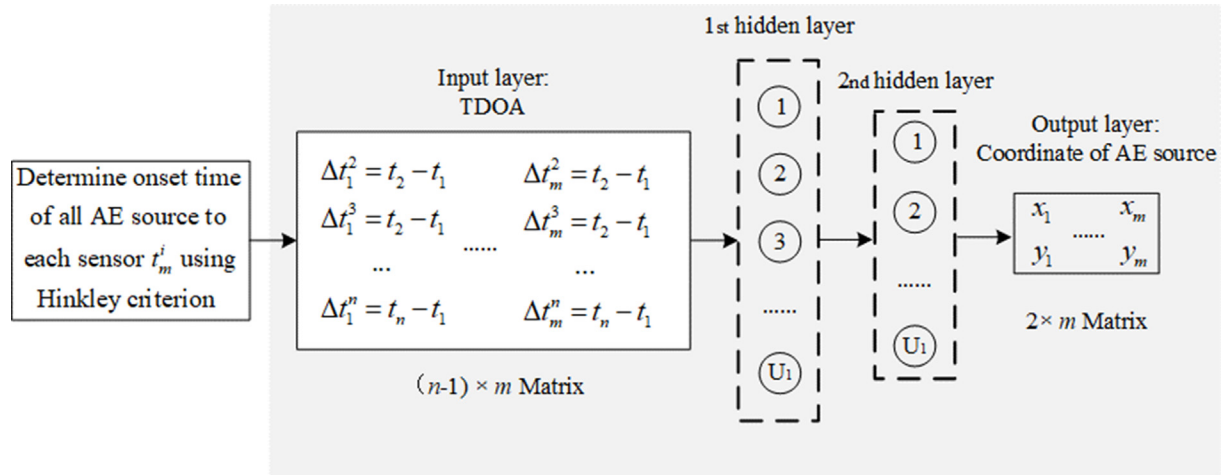
Fig. 23. Source localization method based on ANN.
