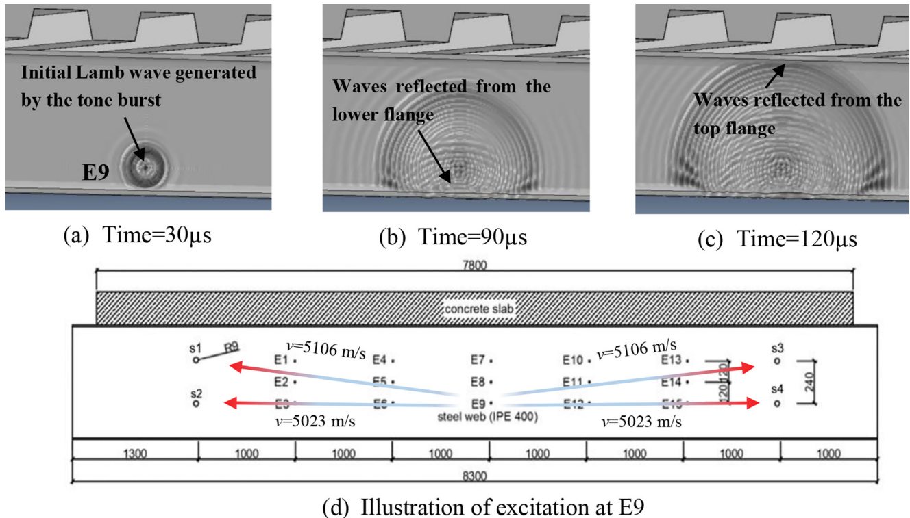
Fig. 13. Simulation of Lamb wave propagation in the girder.
